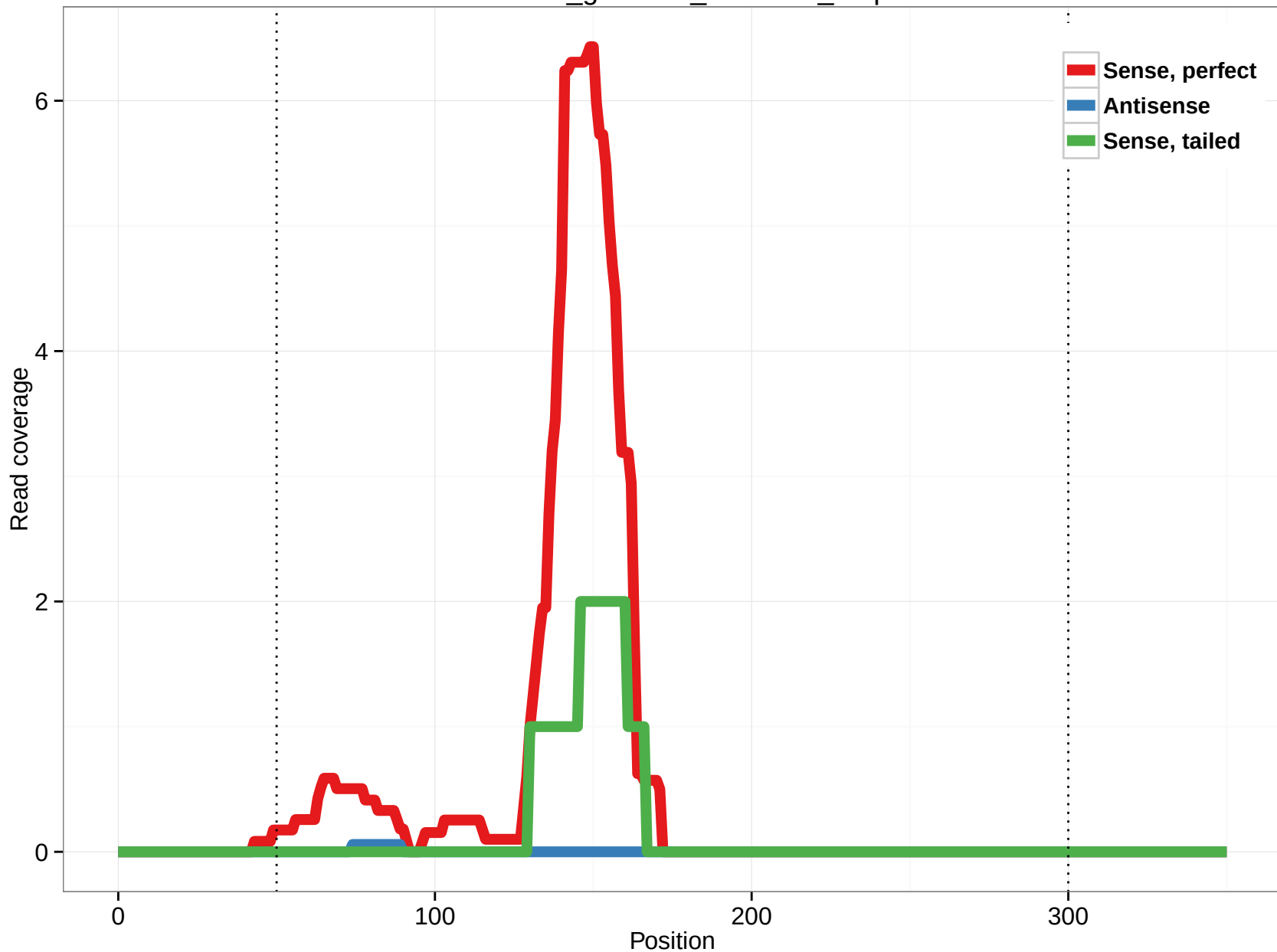
rheMac3_genscan_chr1.736_1.5p
