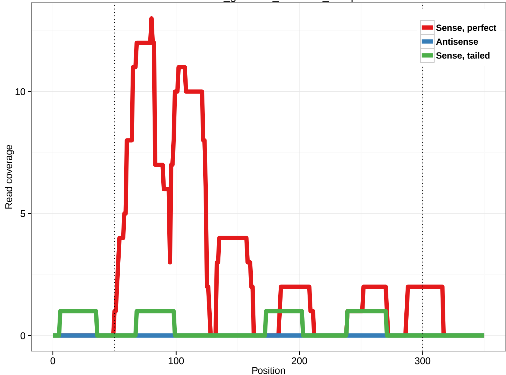
rheMac3_genscan_chr1.728_21.3p
