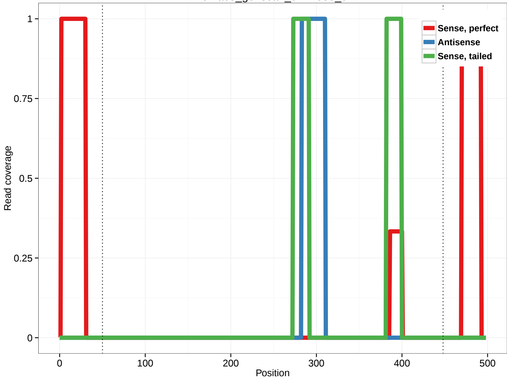
rheMac3_genscan_chr1.685_97
