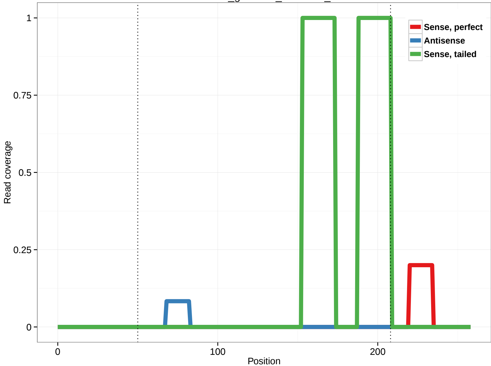
rheMac3_genscan_chr1.685_43
