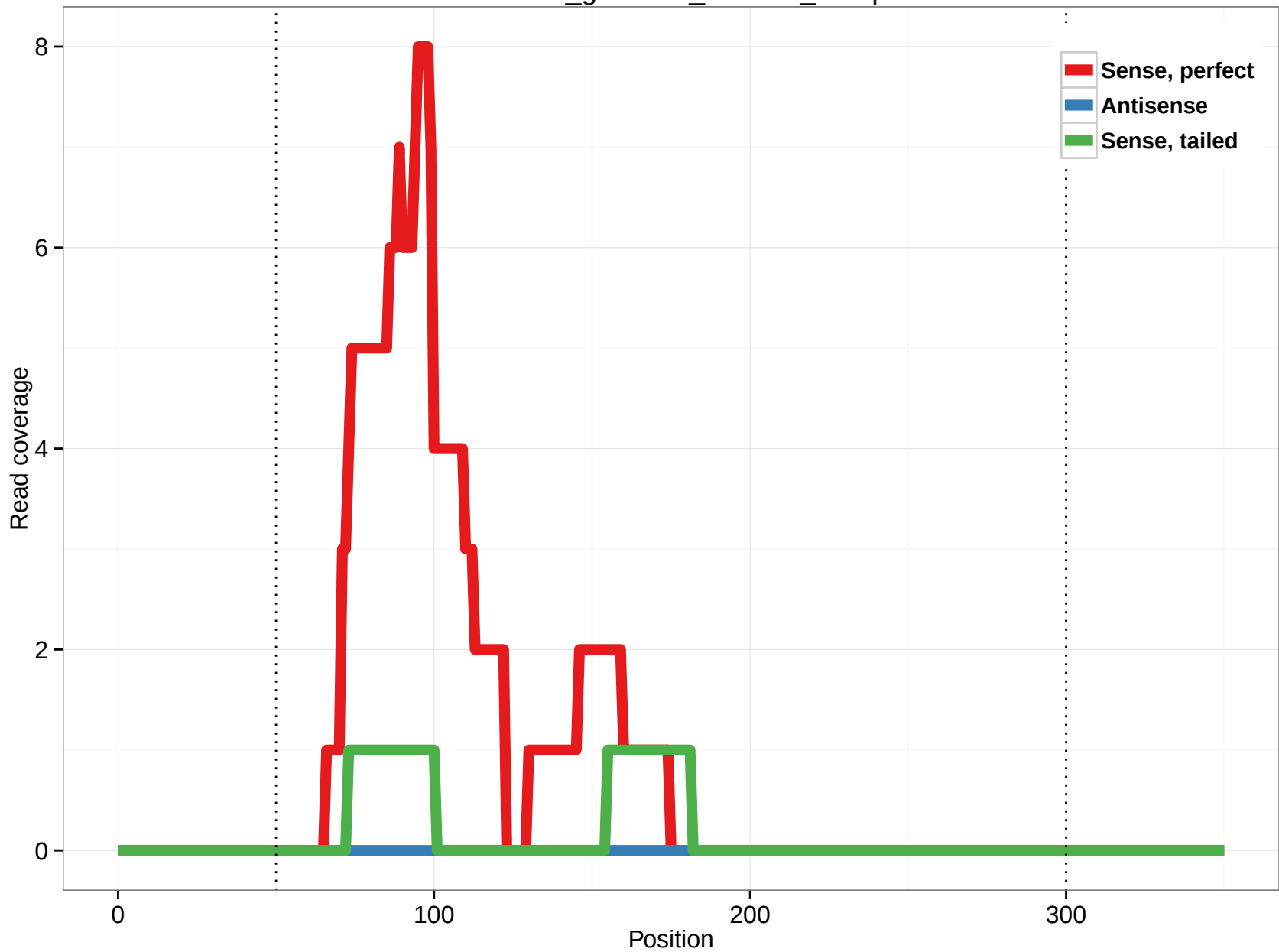
rheMac3_genscan_chr1.67_17.3p
