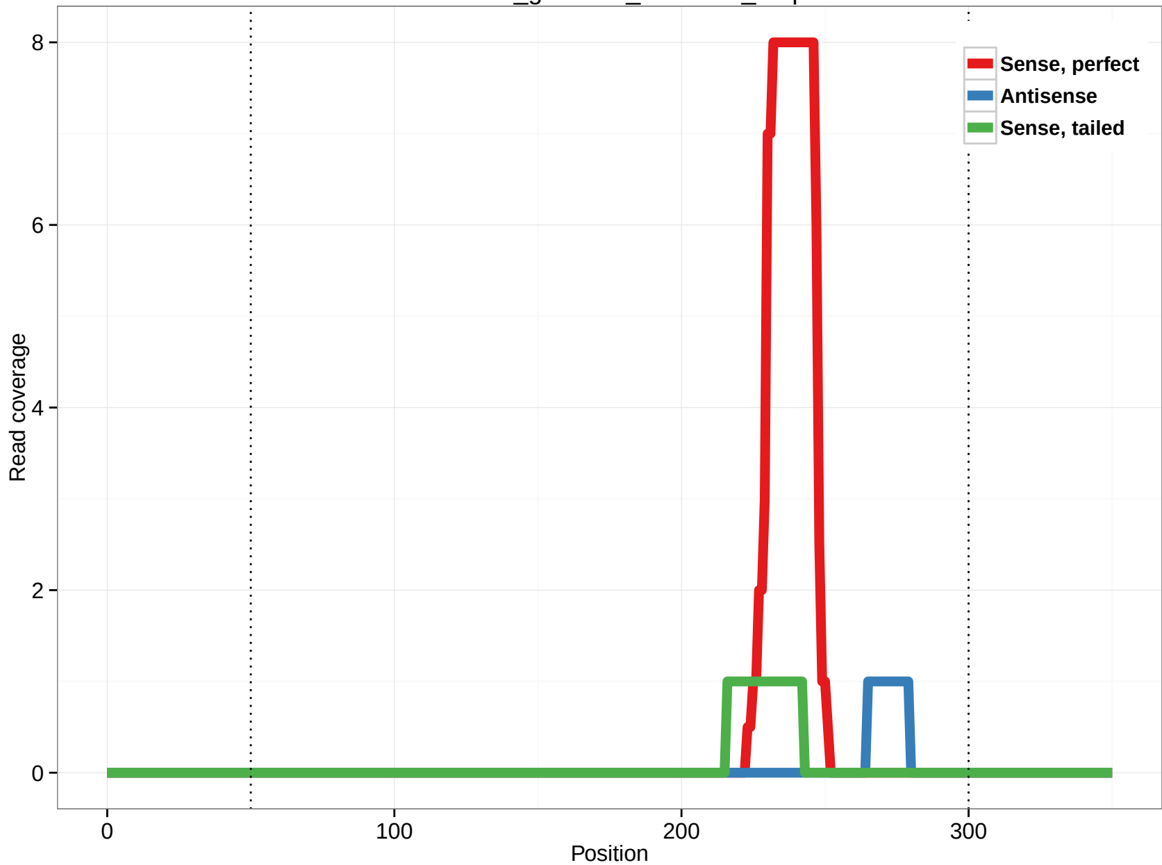
rheMac3_genscan_chr1.664_0.3p
