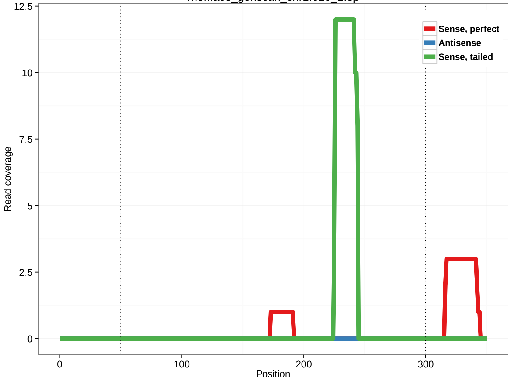
rheMac3_genscan_chr1.626_1.3p
