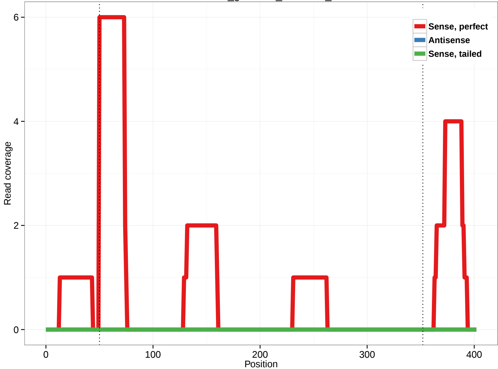
rheMac3_genscan_chr1.622_2
