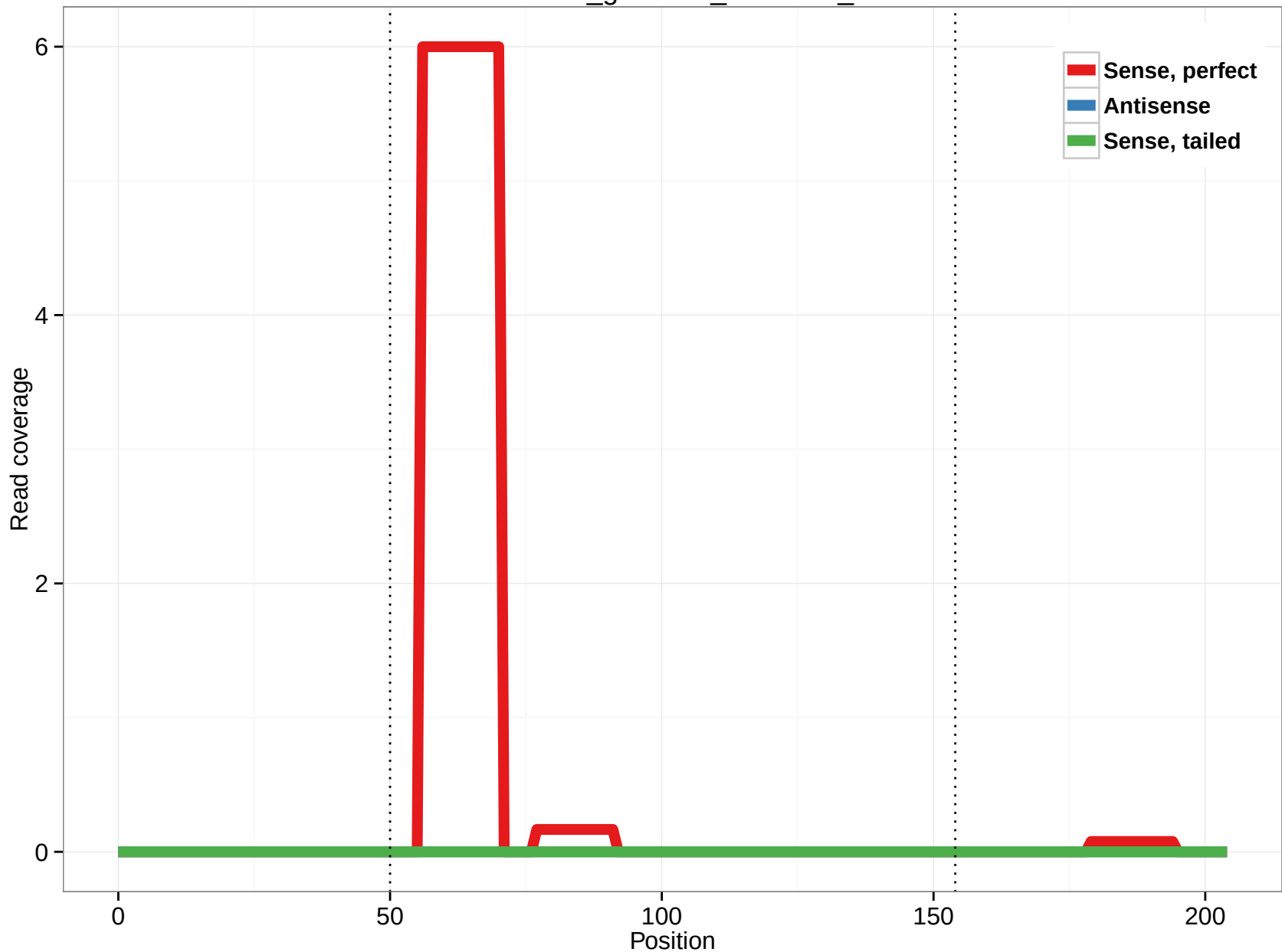
rheMac3_genscan_chr1.575_9
