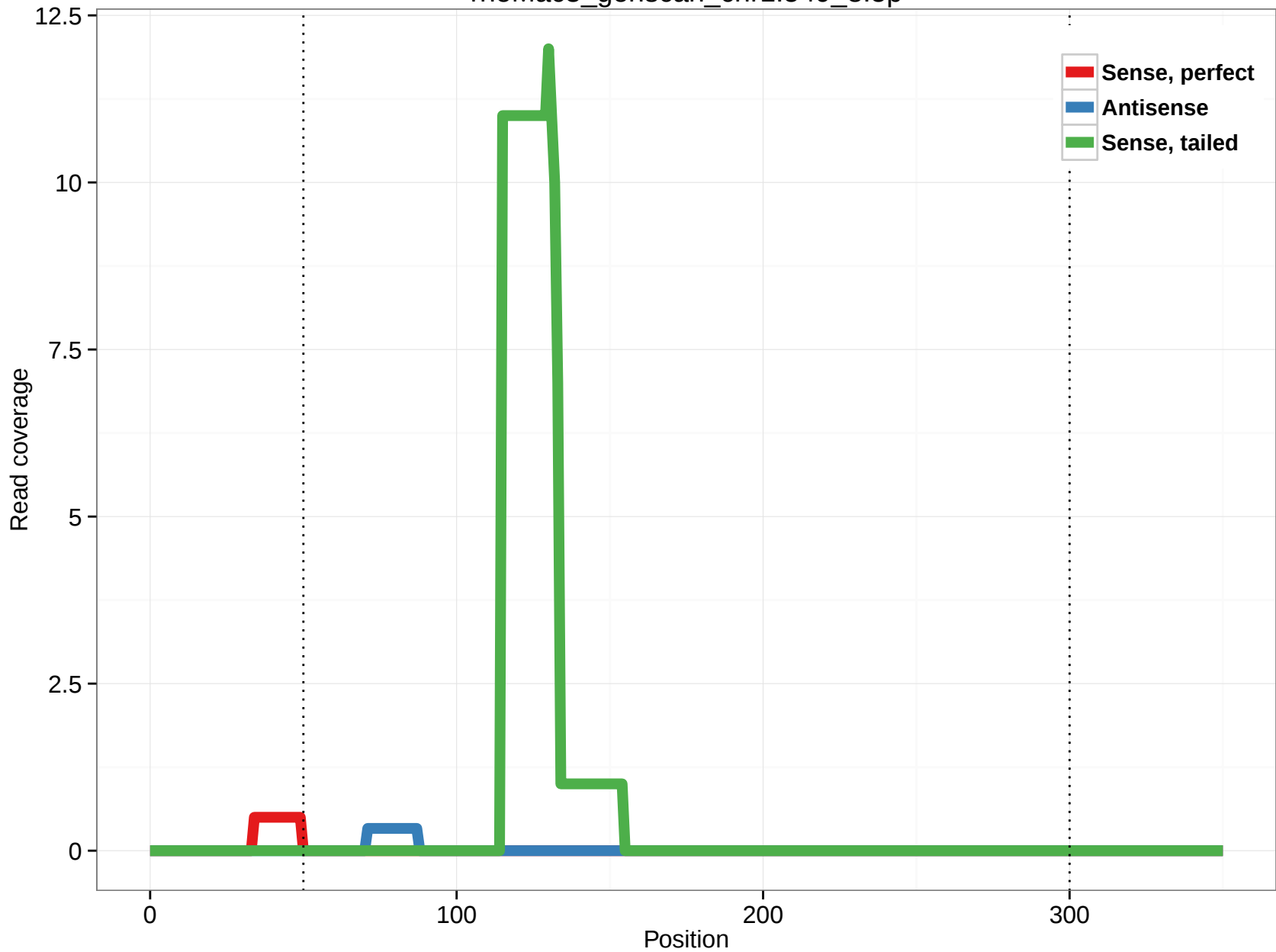
rheMac3_genscan_chr1.549_8.5p
