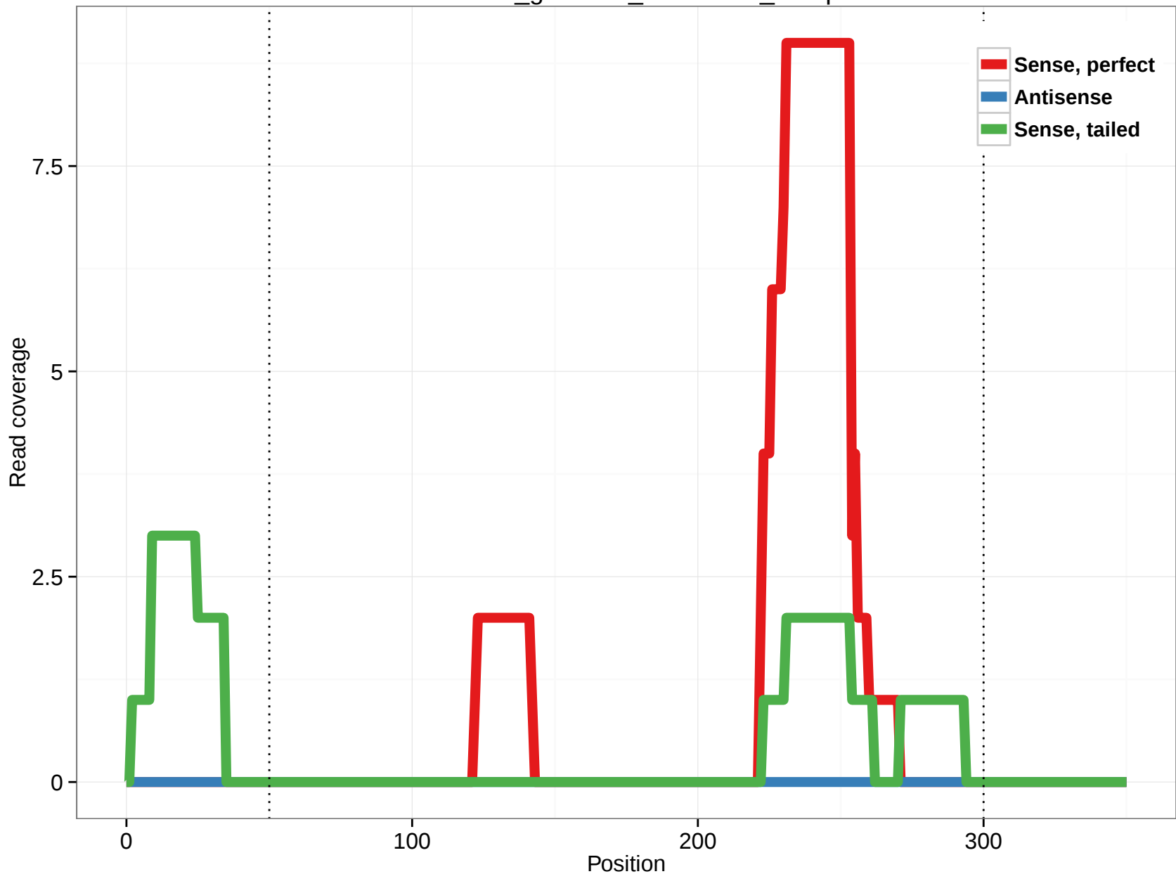
rheMac3_genscan_chr1.4702_24.5p
