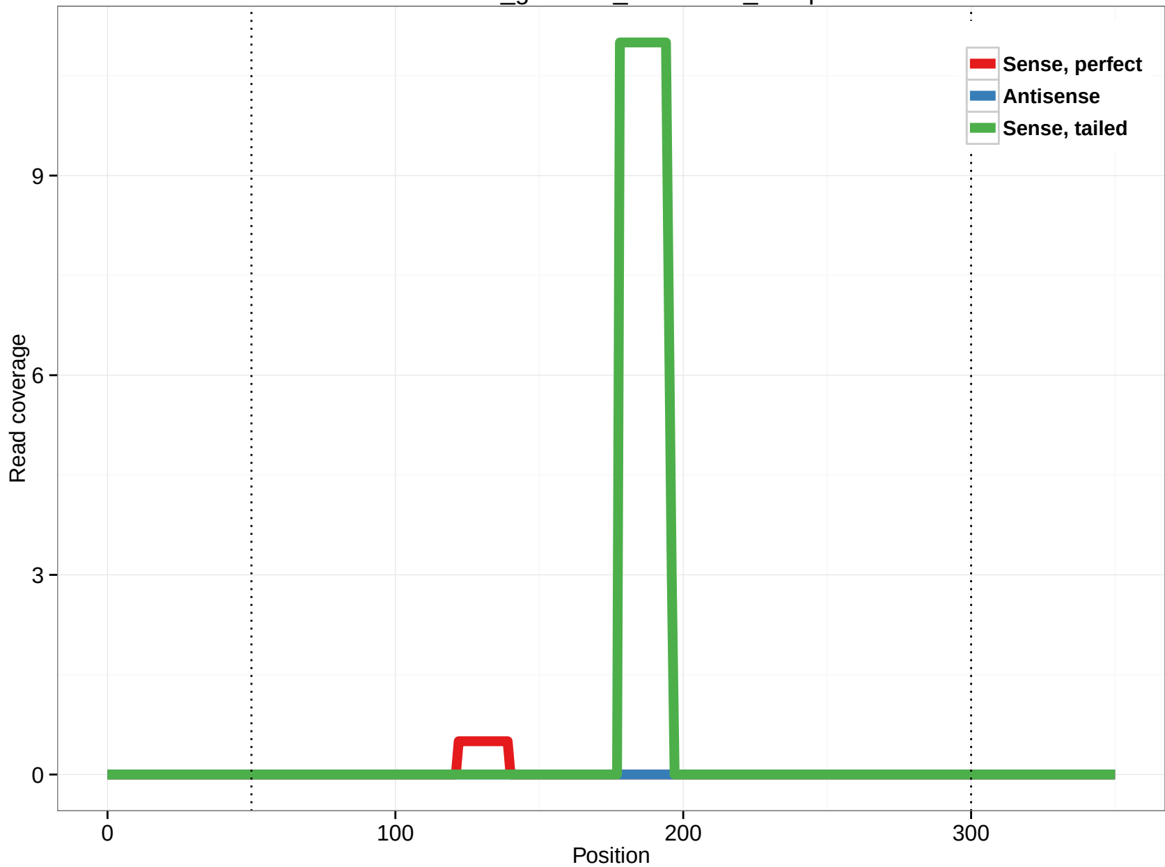
rheMac3_genscan_chr1.4702_14.3p
