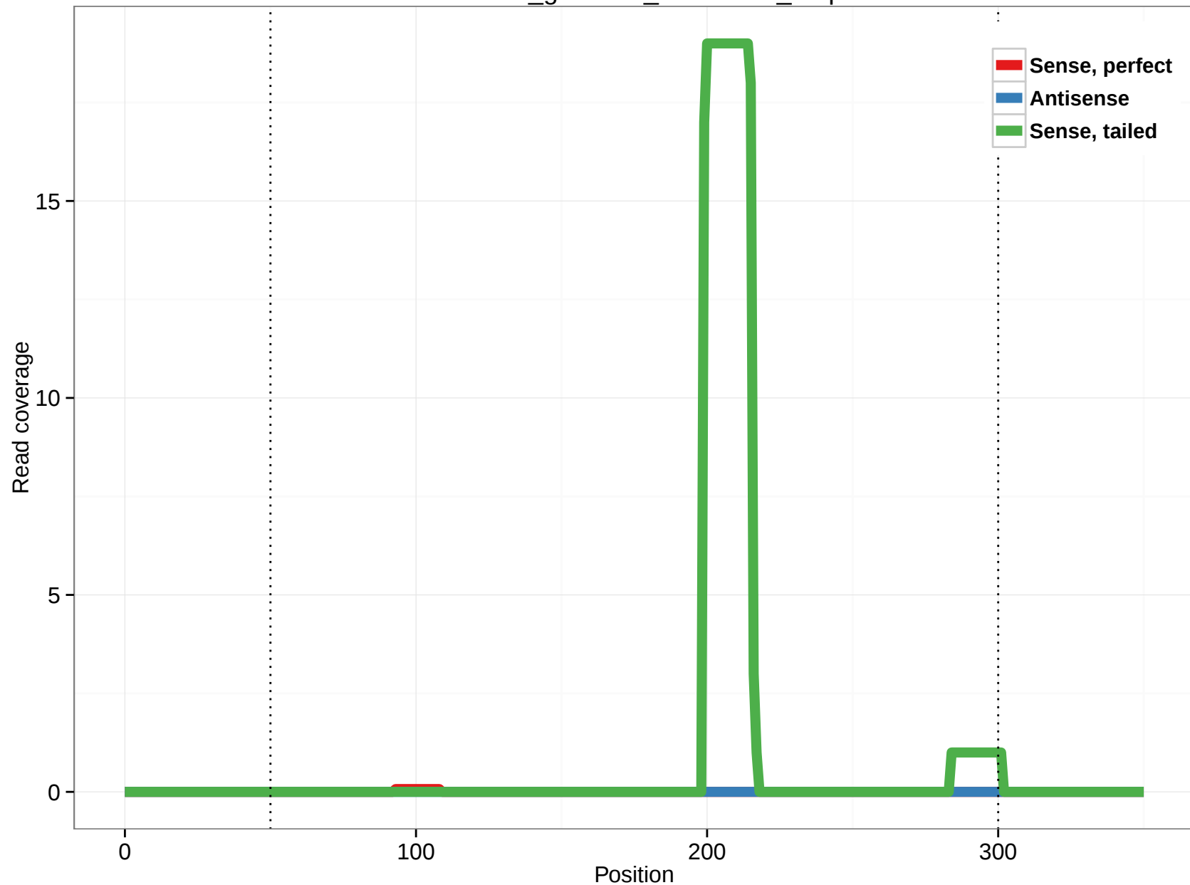
rheMac3_genscan_chr1.4667_7.3p
