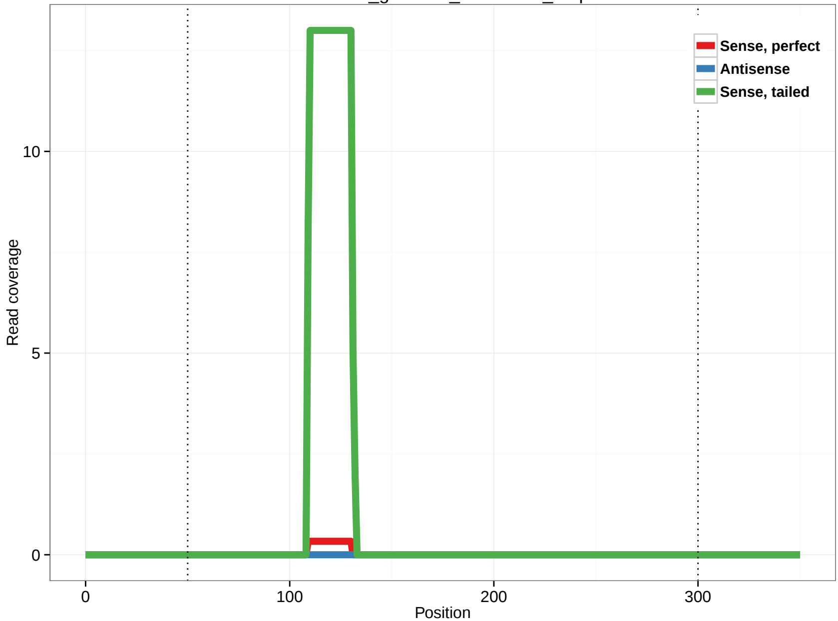
rheMac3_genscan_chr1.4667_5.5p
