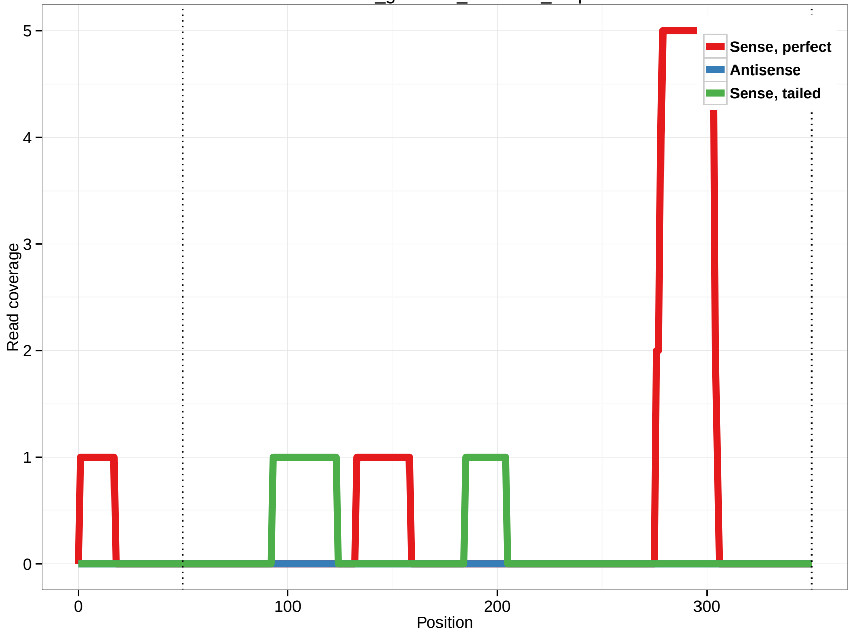
rheMac3_genscan_chr1.465_3.5p
