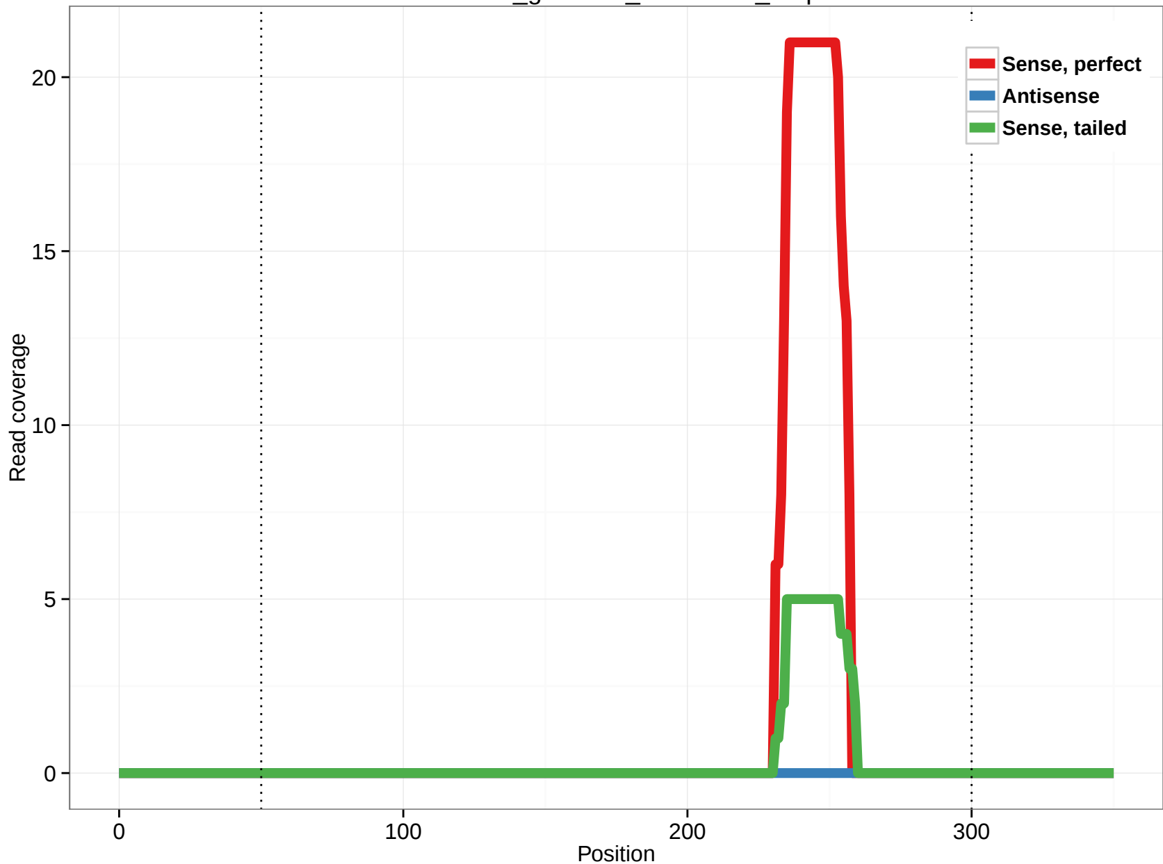
rheMac3_genscan_chr1.4633_3.3p
