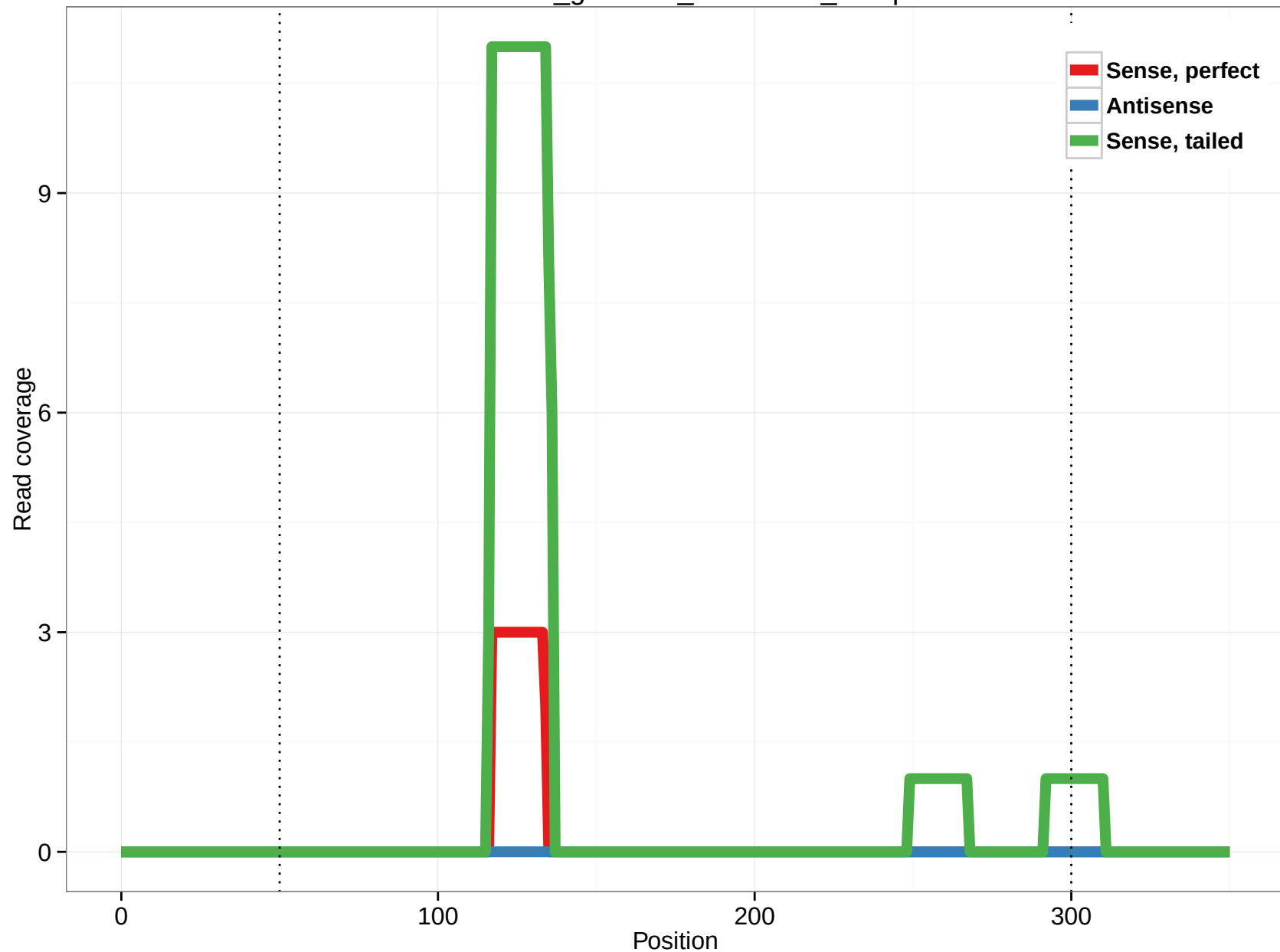
rheMac3_genscan_chr1.4582_10.5p
