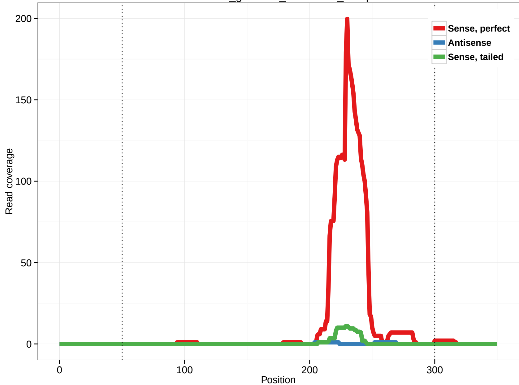
rheMac3_genscan_chr1.4577_10.3p
