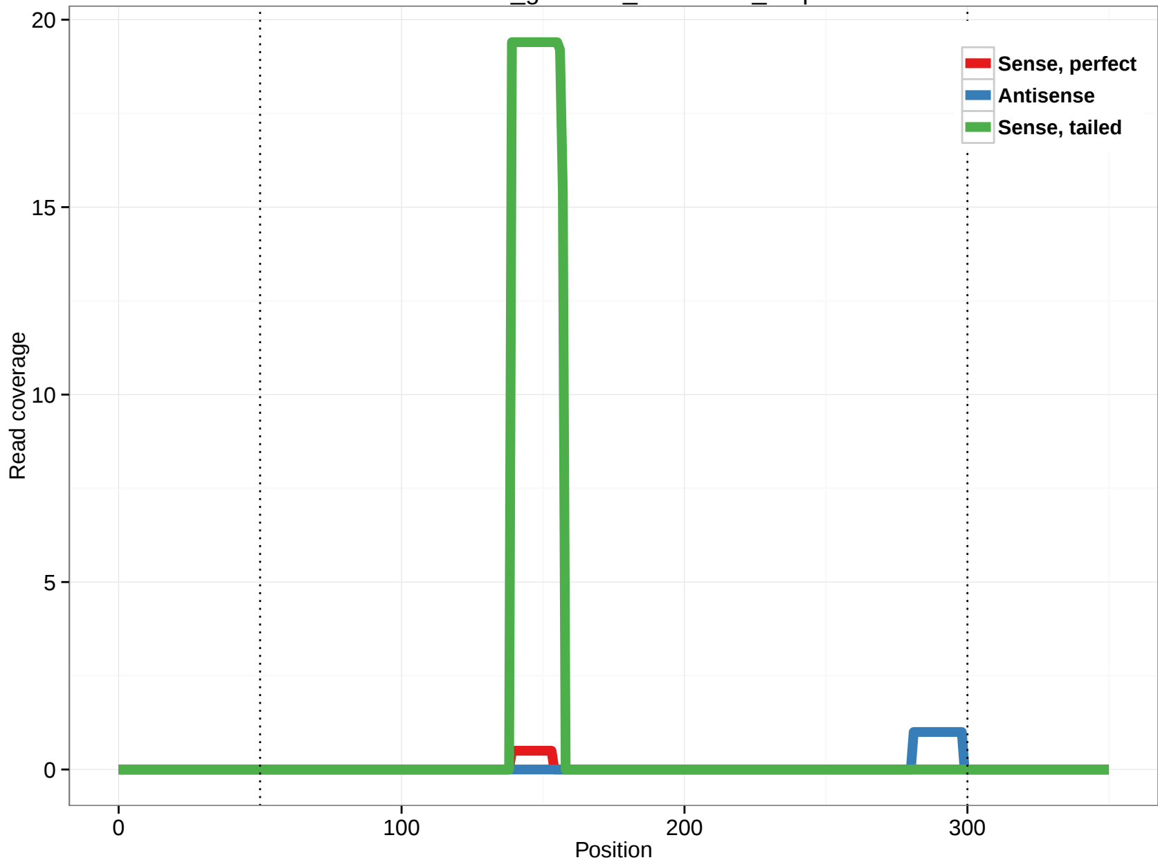
rheMac3_genscan_chr1.4533_3.3p
