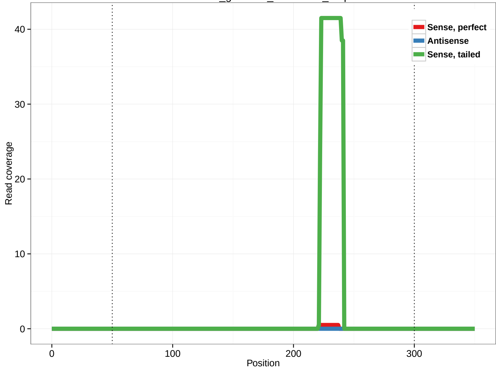
rheMac3_genscan_chr1.4482_6.5p
