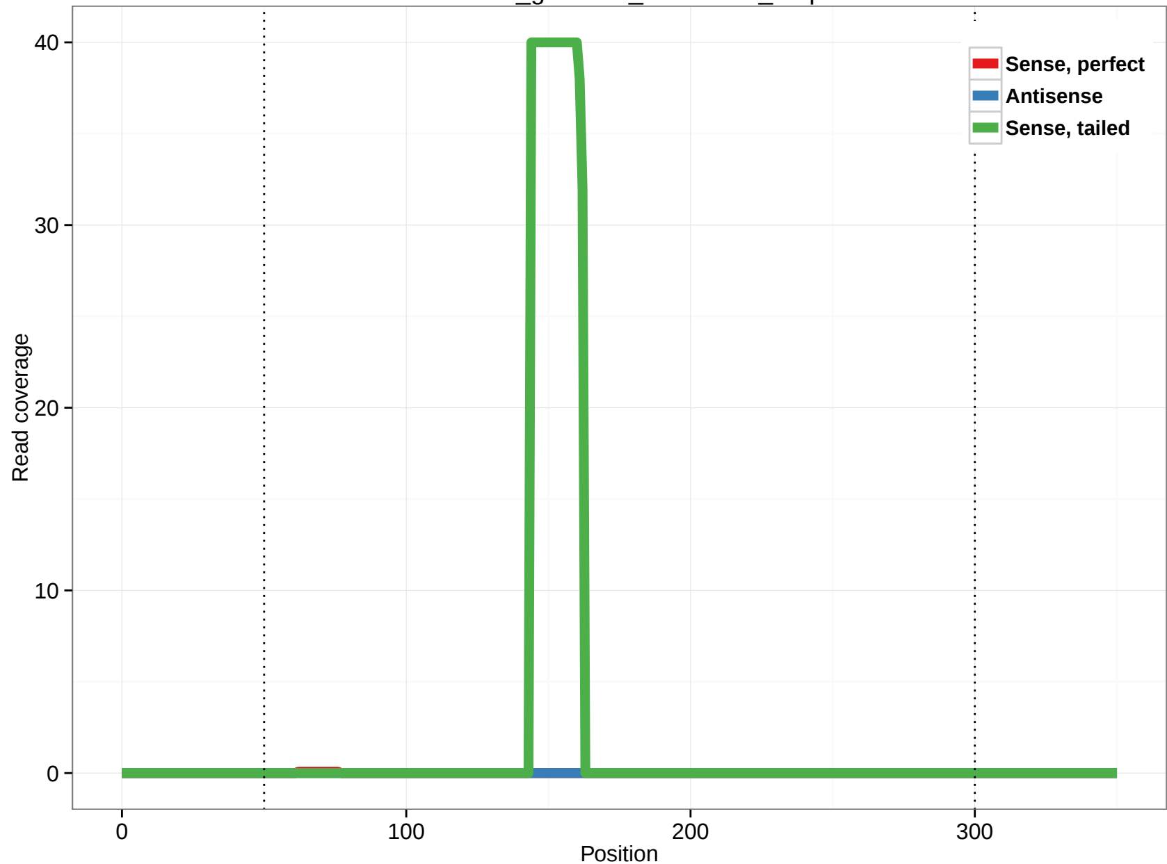
rheMac3_genscan_chr1.4451_7.3p
