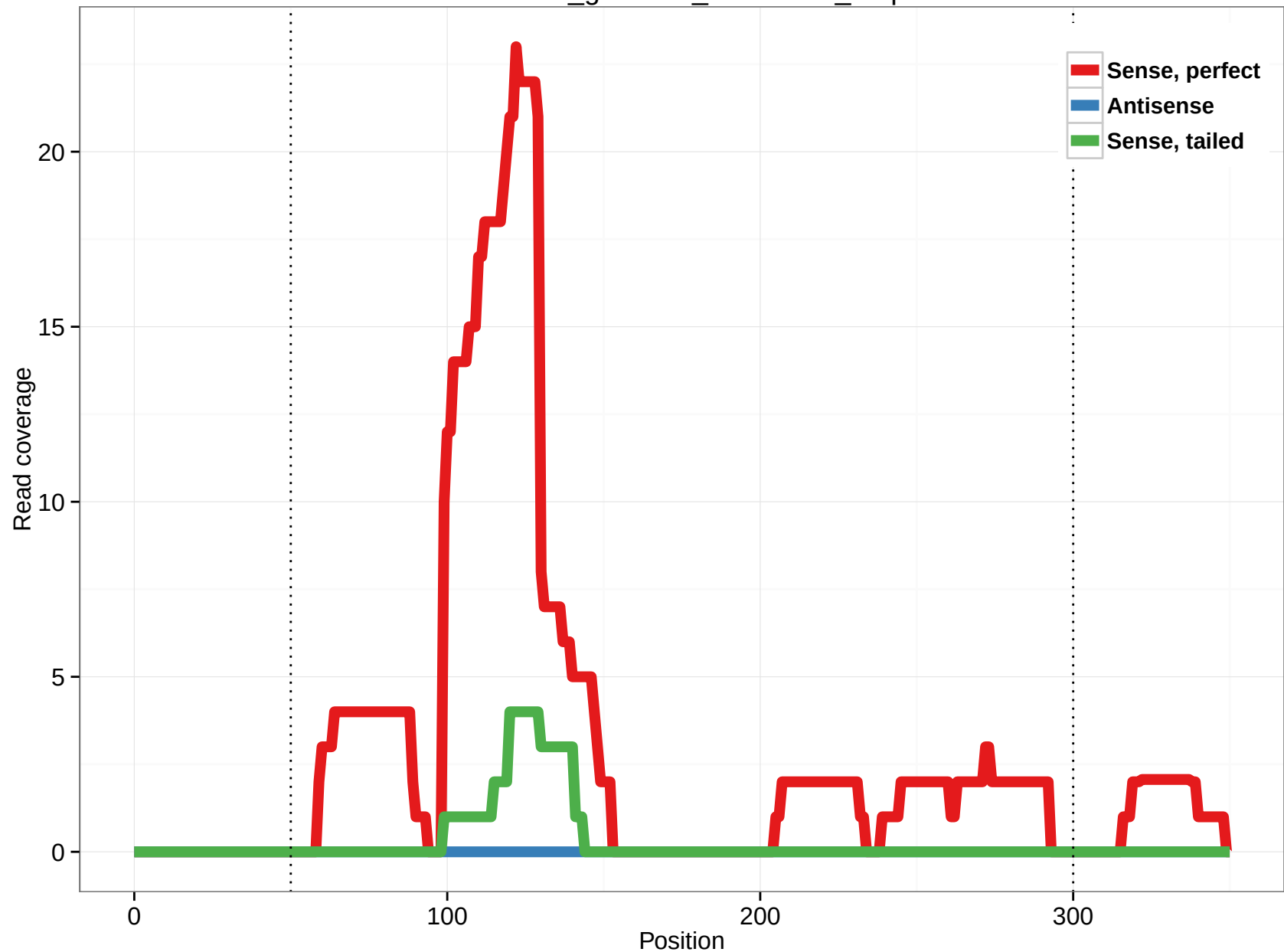
rheMac3_genscan_chr1.4375_8.5p
