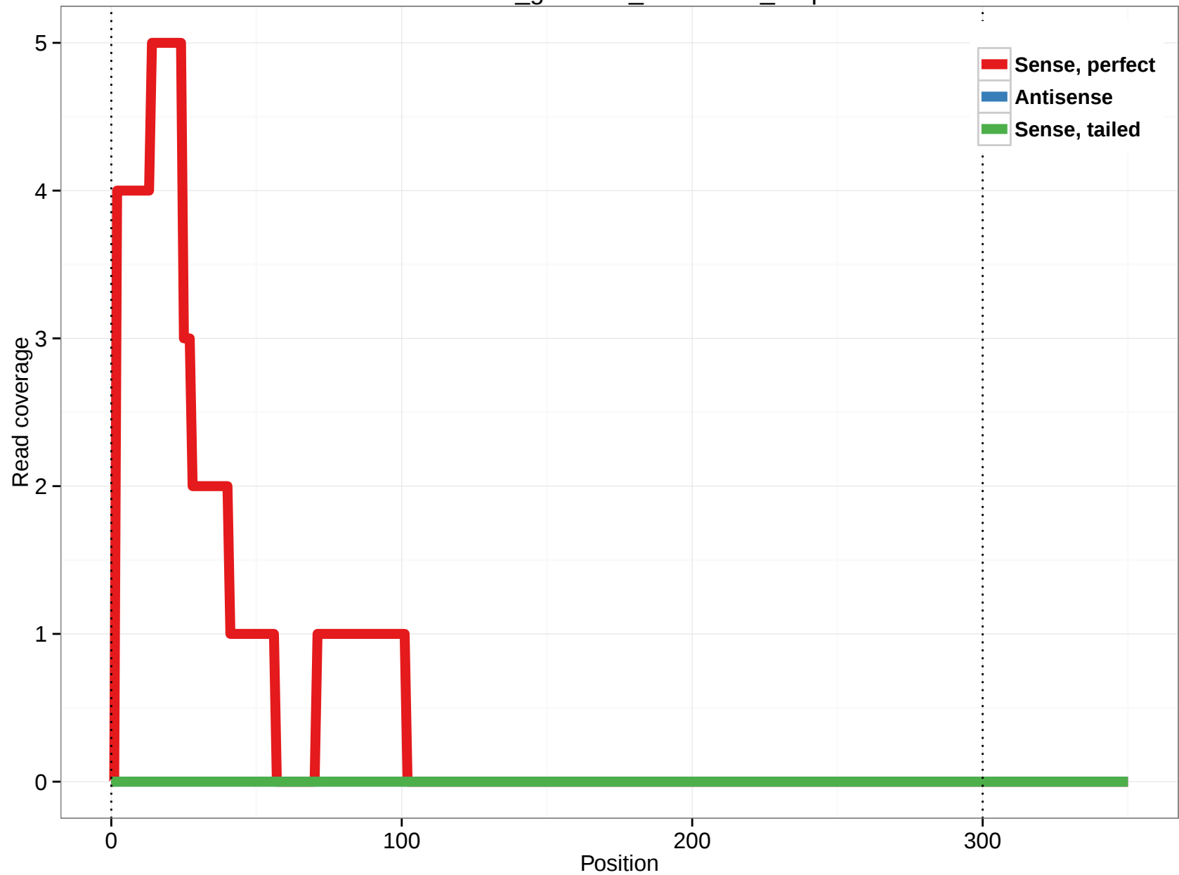
rheMac3_genscan_chr1.4370_0.3p
