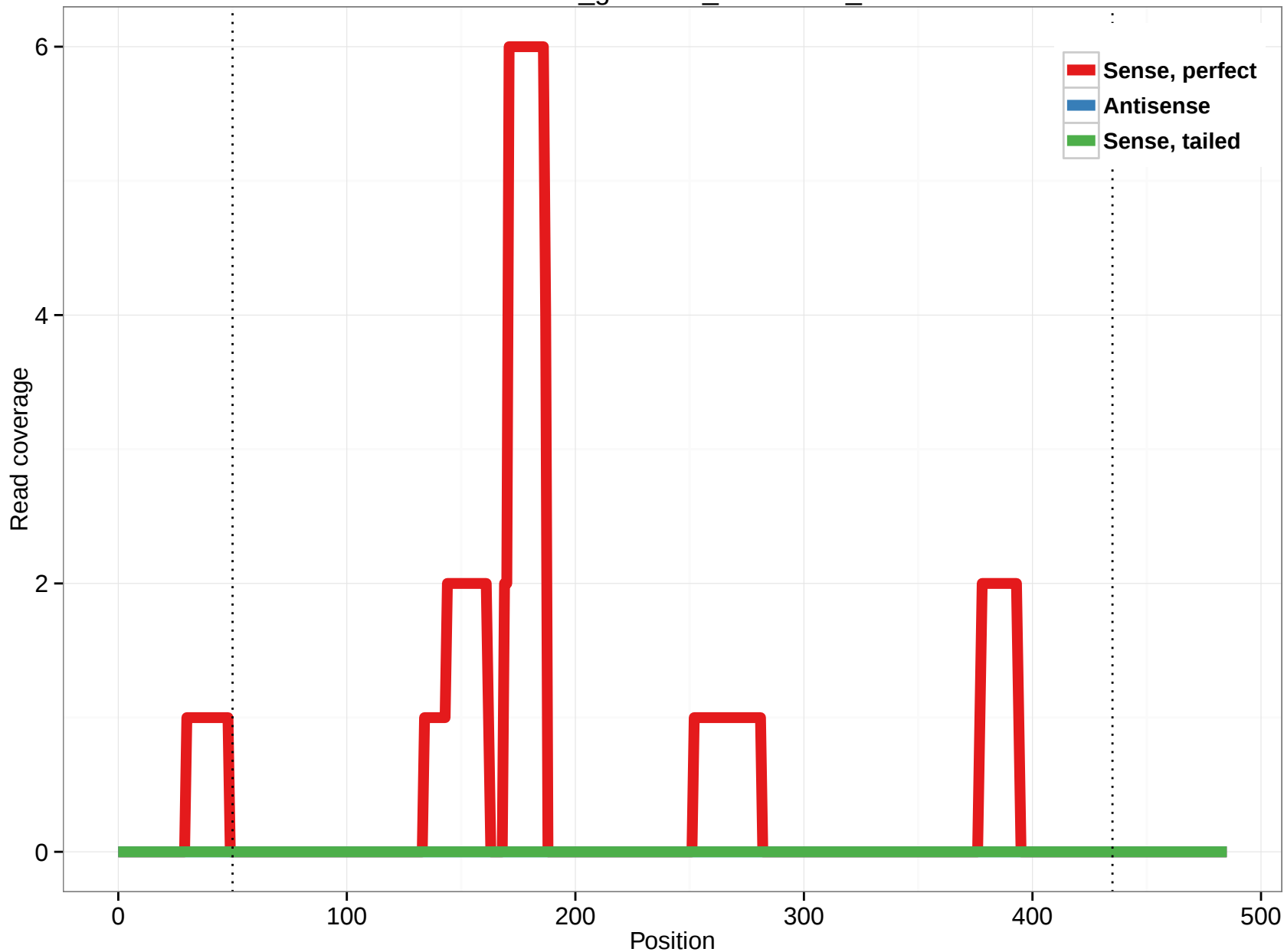
rheMac3_genscan_chr1.4117_2
