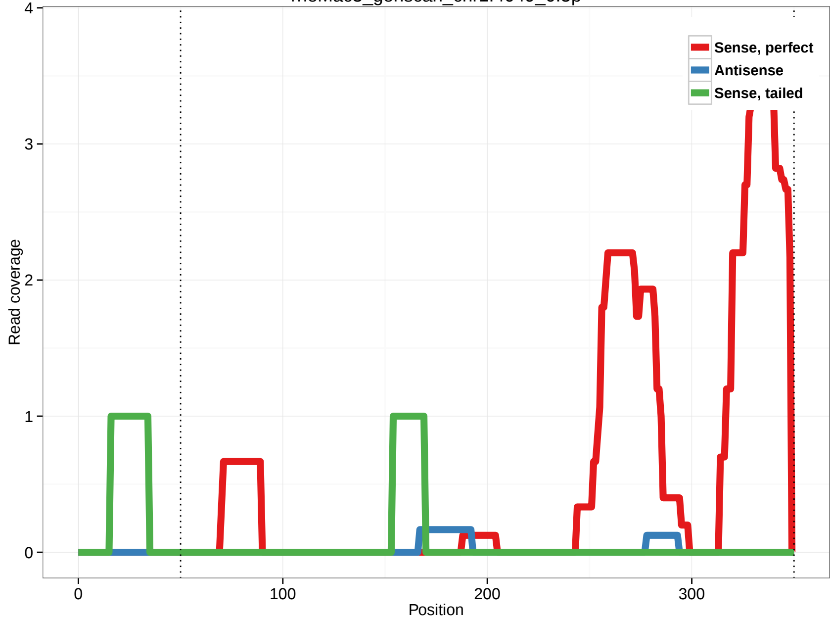
rheMac3_genscan_chr1.4049_0.5p
