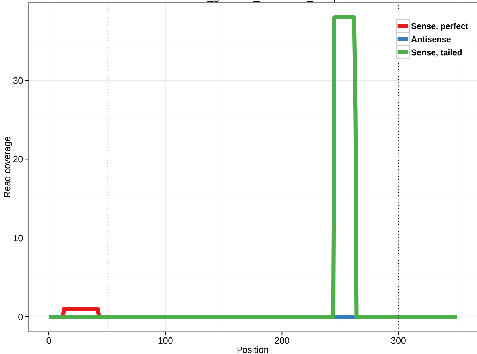
rheMac3_genscan_chr1.4035_10.5p
