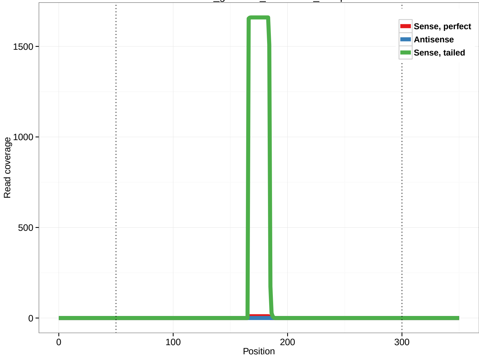
rheMac3_genscan_chr1.4004_13.5p
