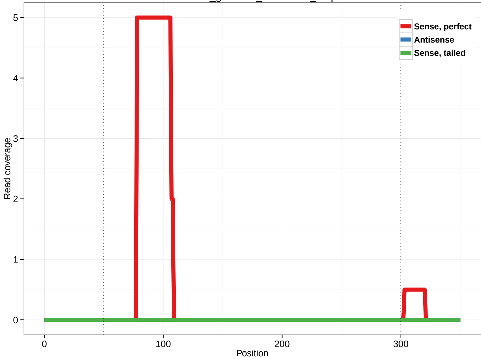
rheMac3_genscan_chr1.3957_7.5p
