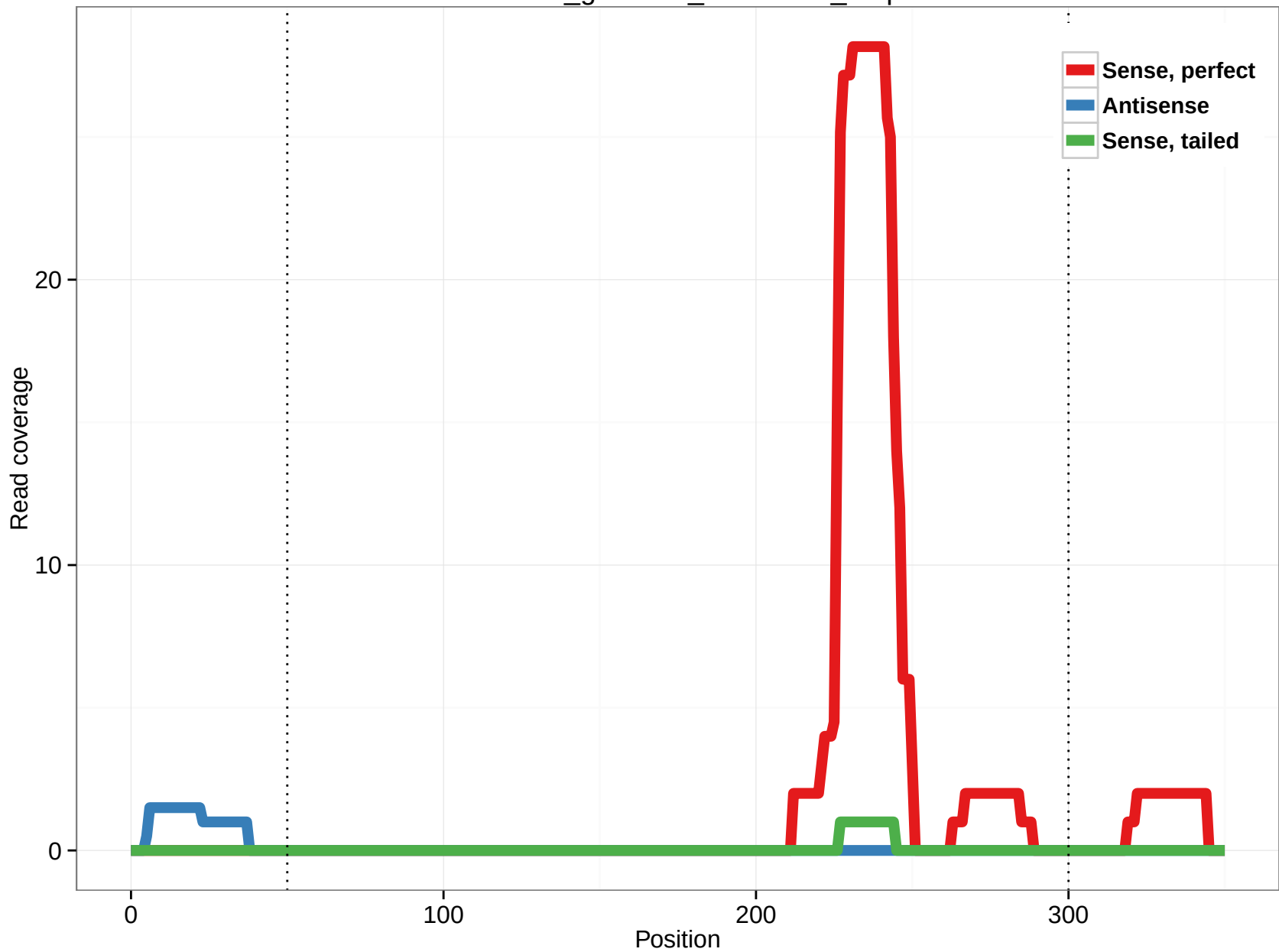
rheMac3_genscan_chr1.3956_0.3p
