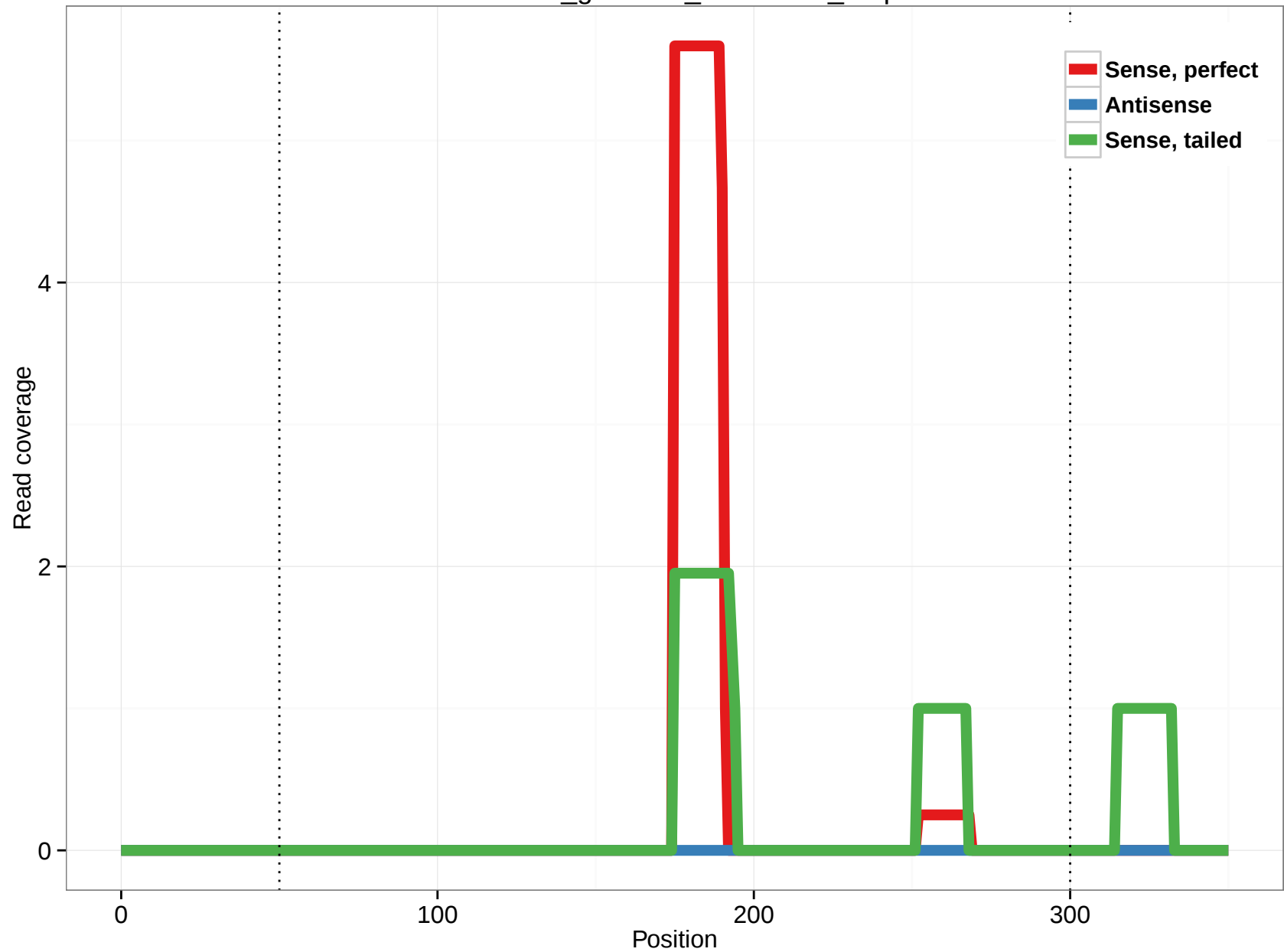
rheMac3_genscan_chr1.3872_5.5p
