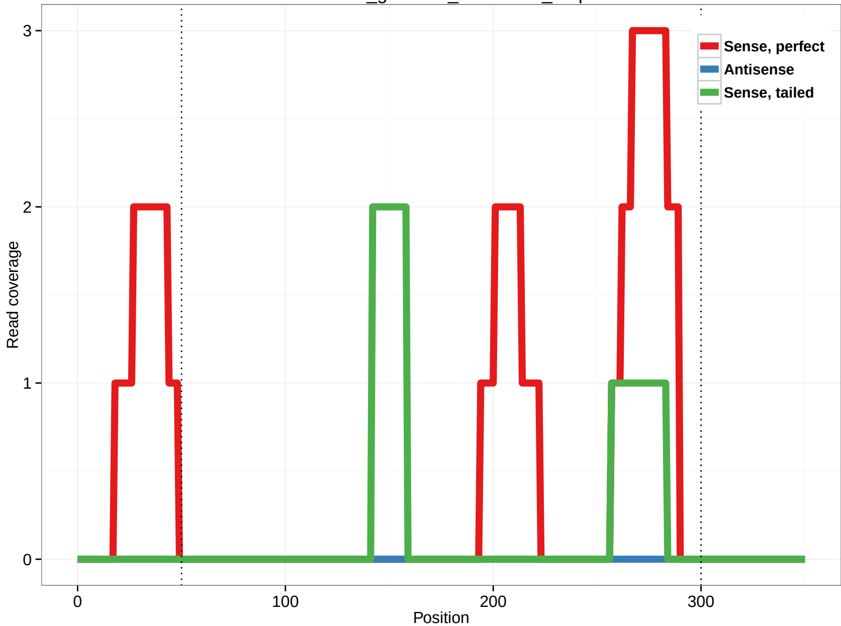
rheMac3_genscan_chr1.3851_3.5p
