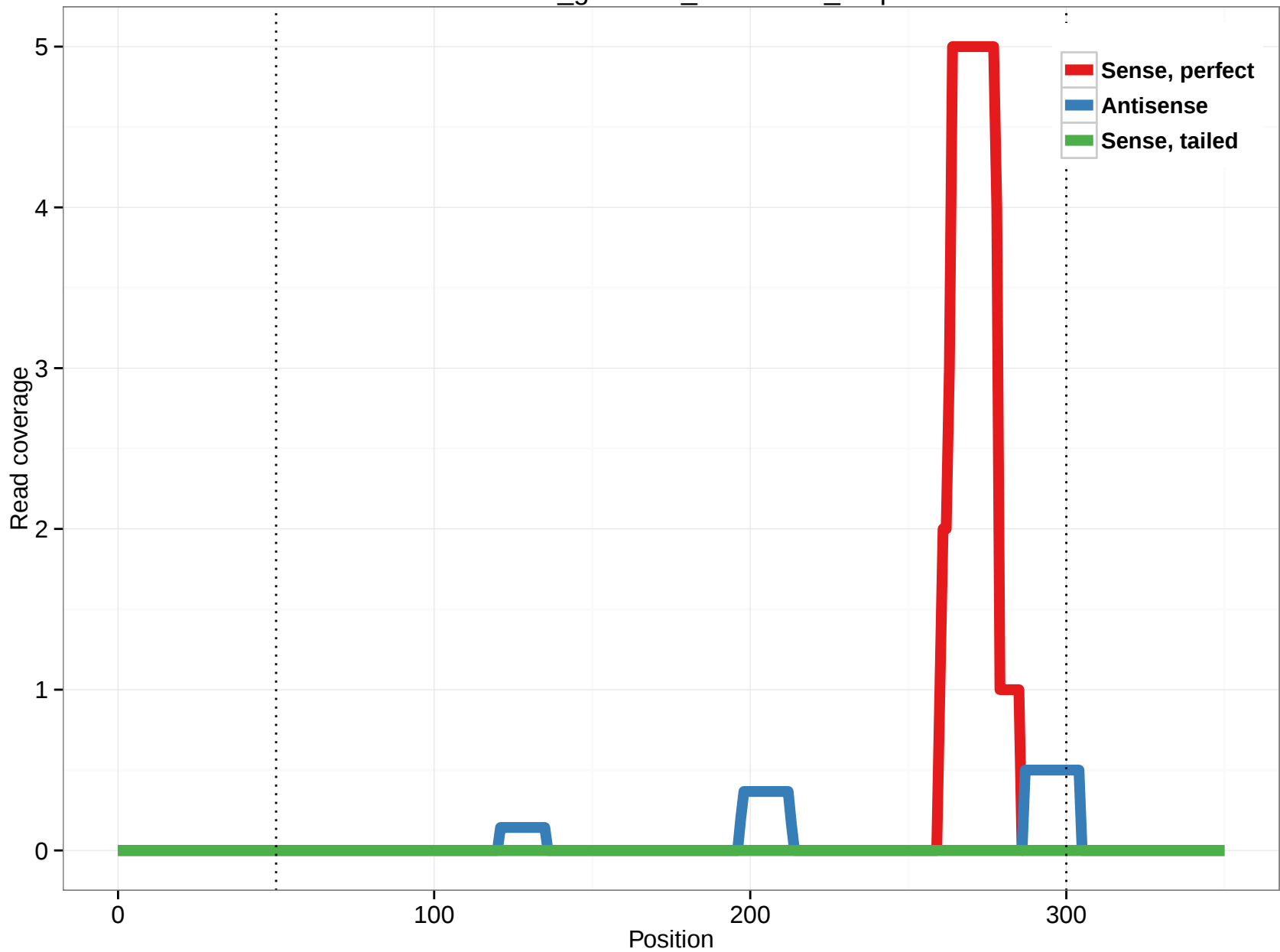
rheMac3_genscan_chr1.3800_2.3p
