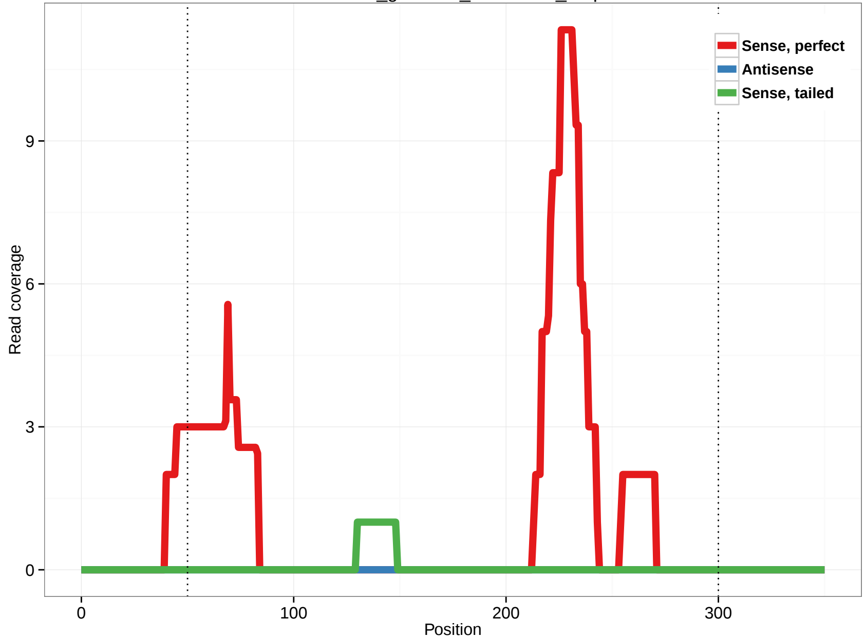
rheMac3_genscan_chr1.3775_1.5p
