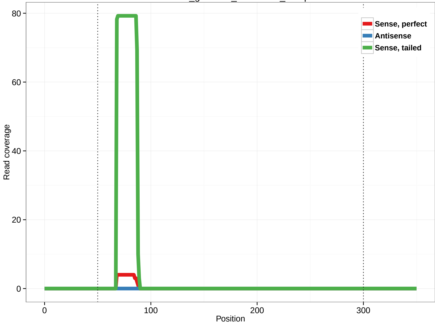
rheMac3_genscan_chr1.3754_15.5p
