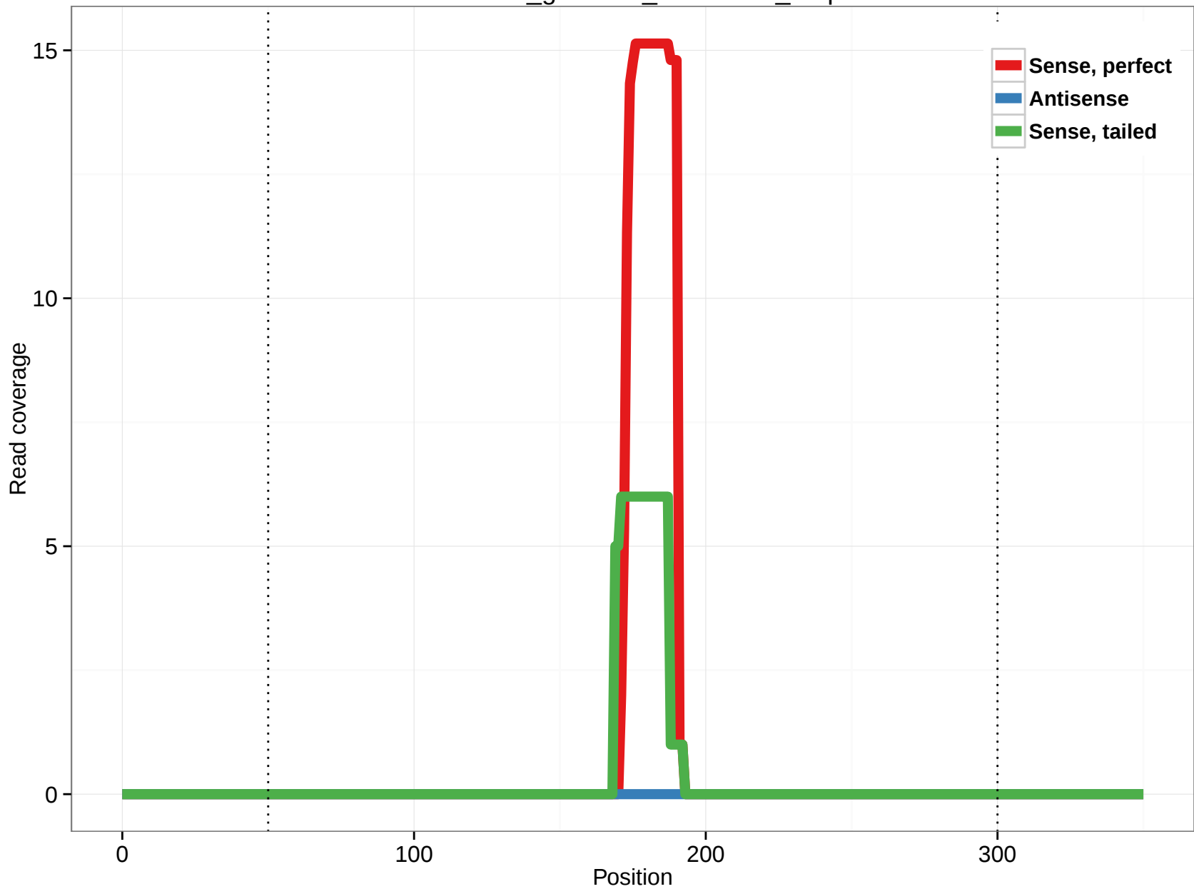
rheMac3_genscan_chr1.3578_1.3p
