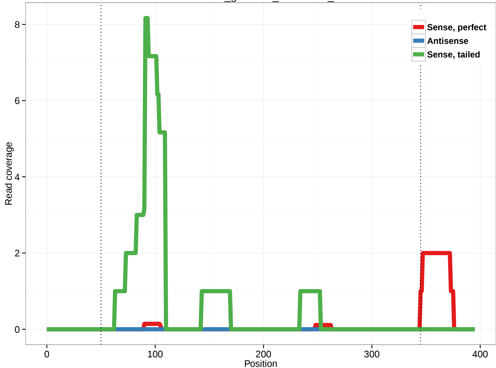
rheMac3_genscan_chr1.3559_5
