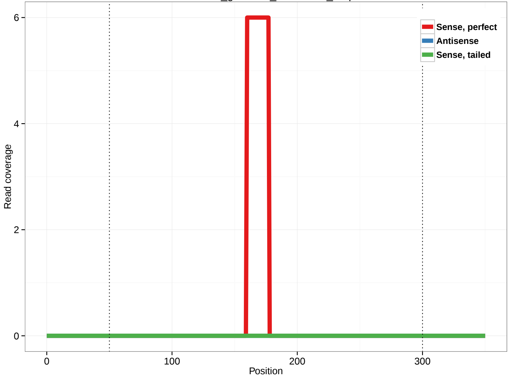
rheMac3_genscan_chr1.3541_1.3p
