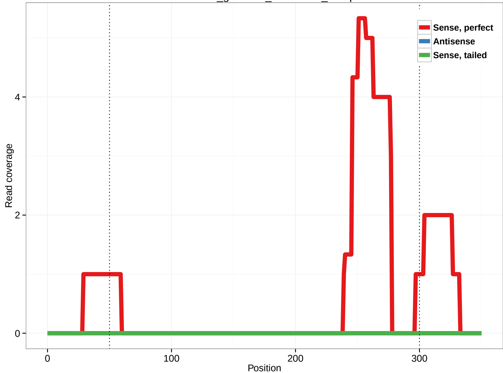
rheMac3_genscan_chr1.3499_11.5p
