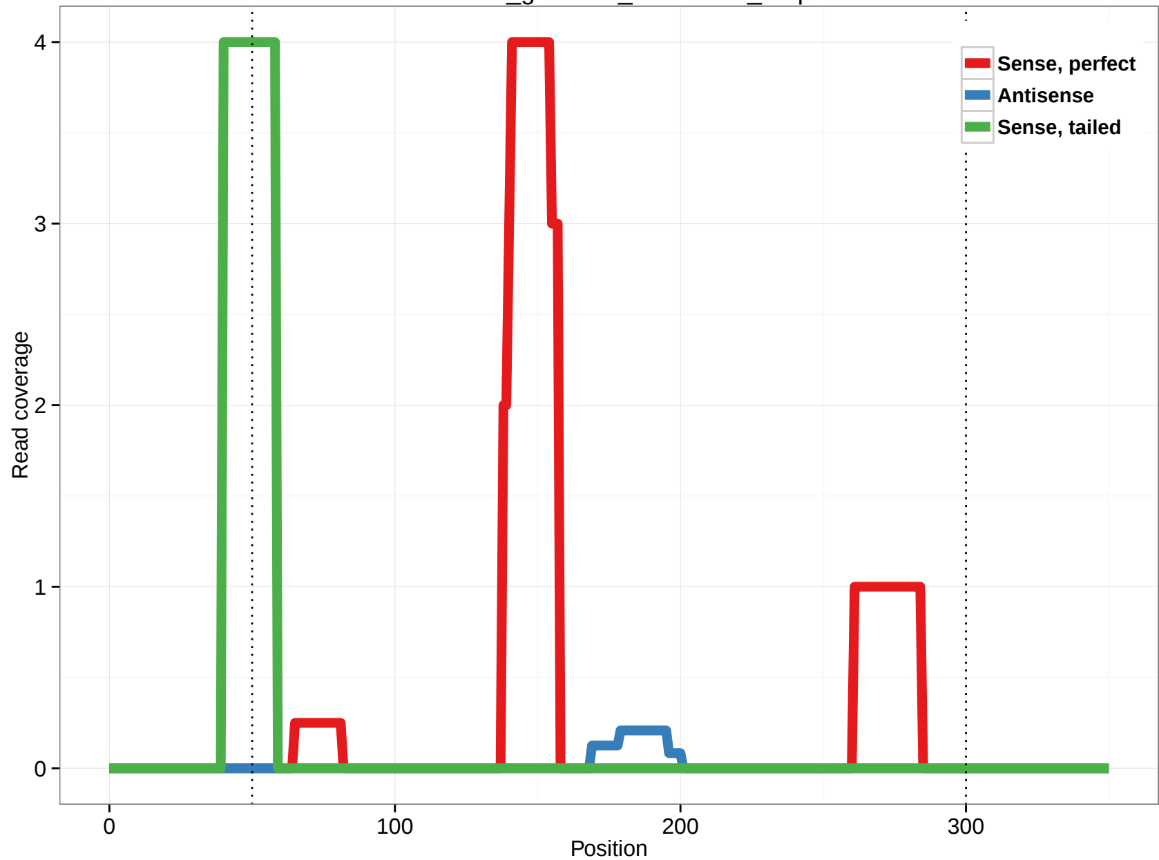
rheMac3_genscan_chr1.3494_6.3p
