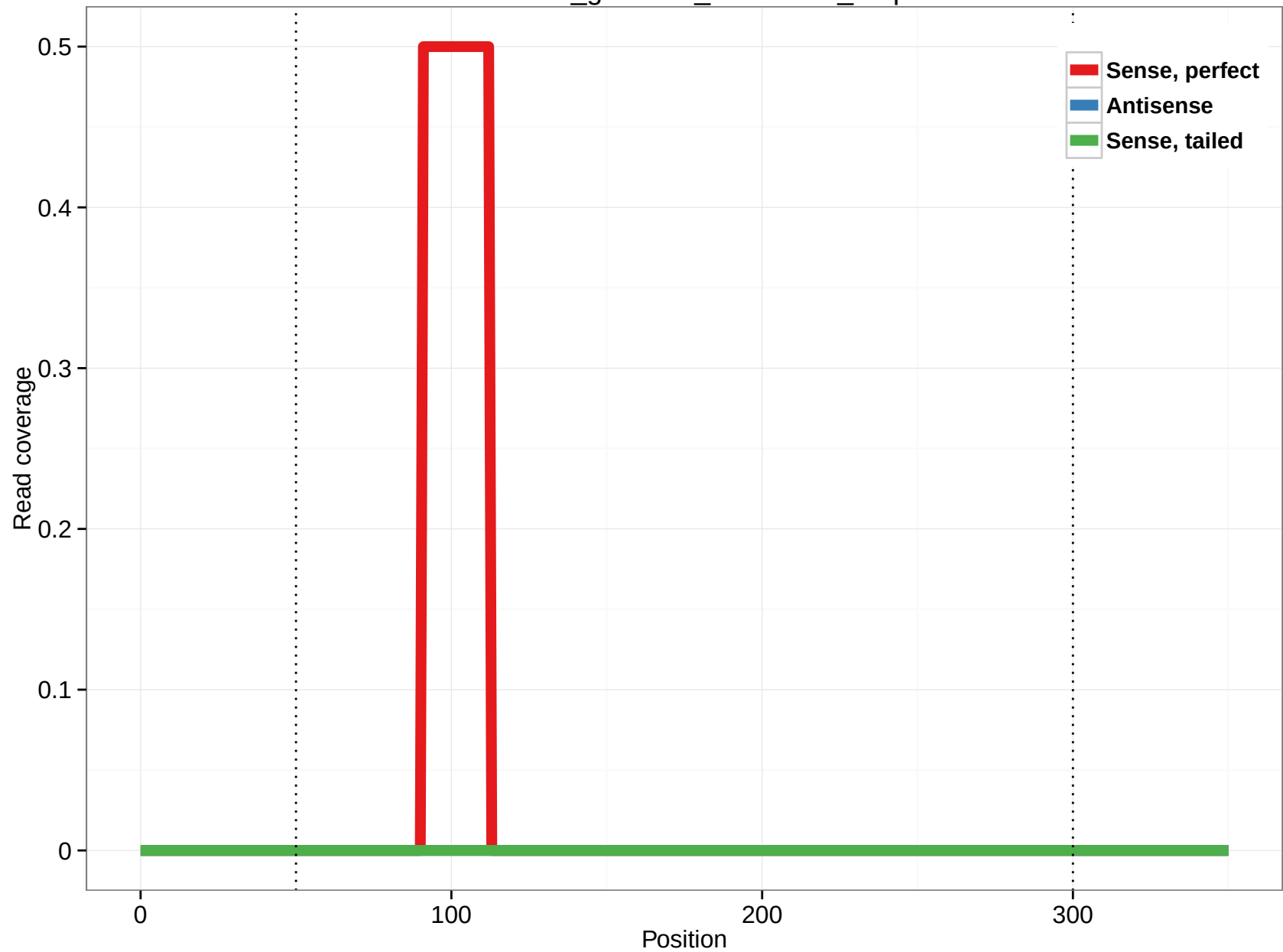
rheMac3_genscan_chr1.3470_1.3p
