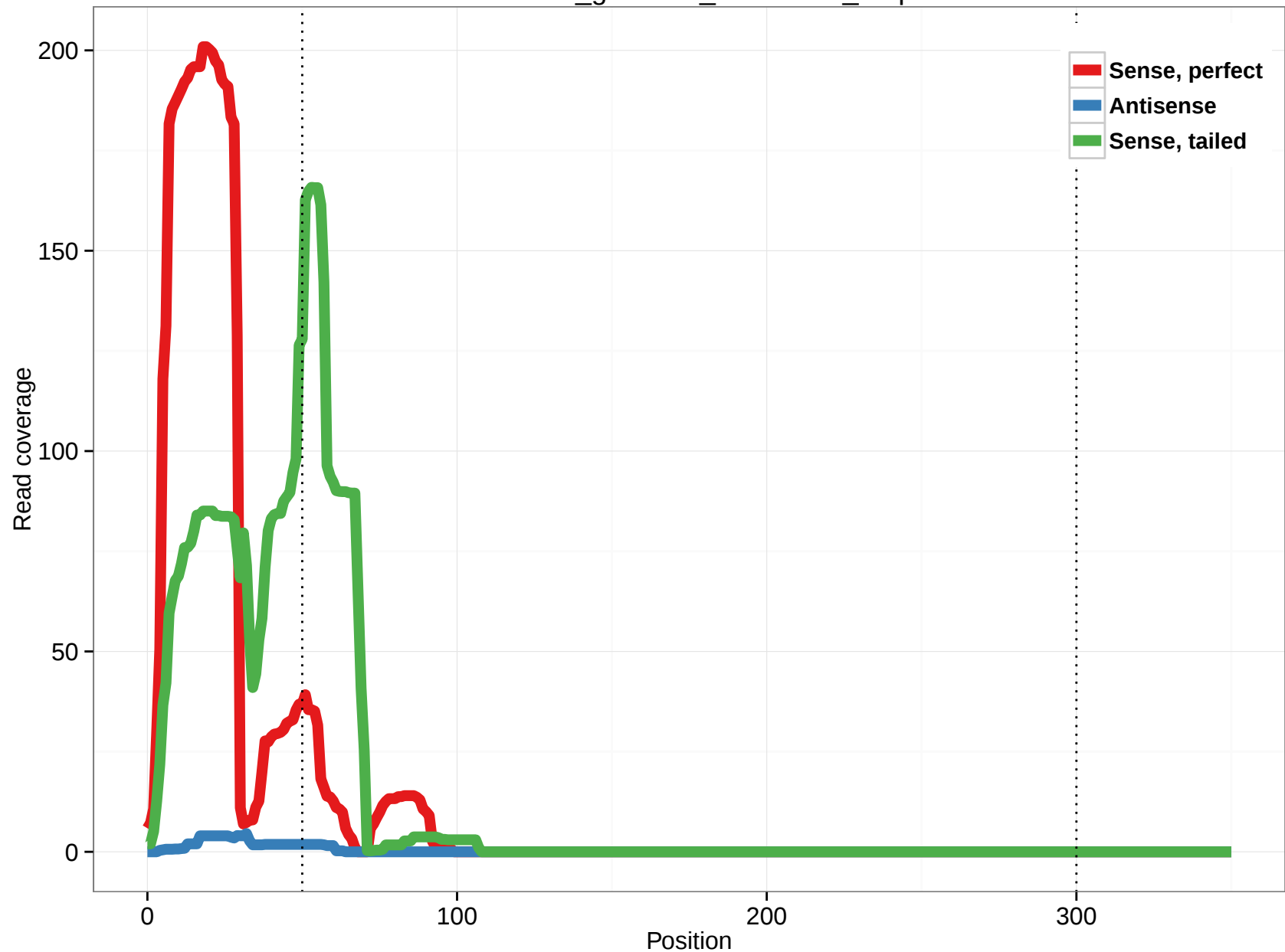
rheMac3_genscan_chr1.3446_1.3p
