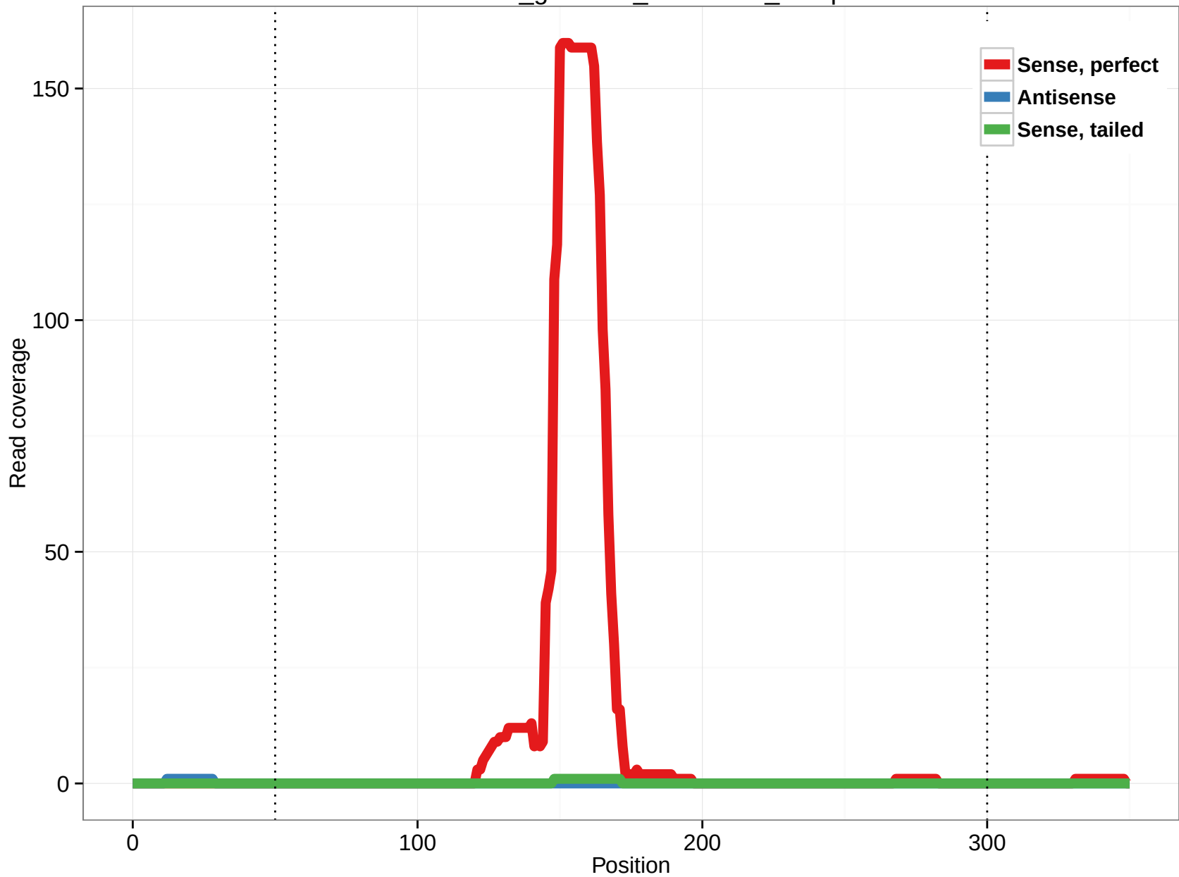
rheMac3_genscan_chr1.3439_19.5p
