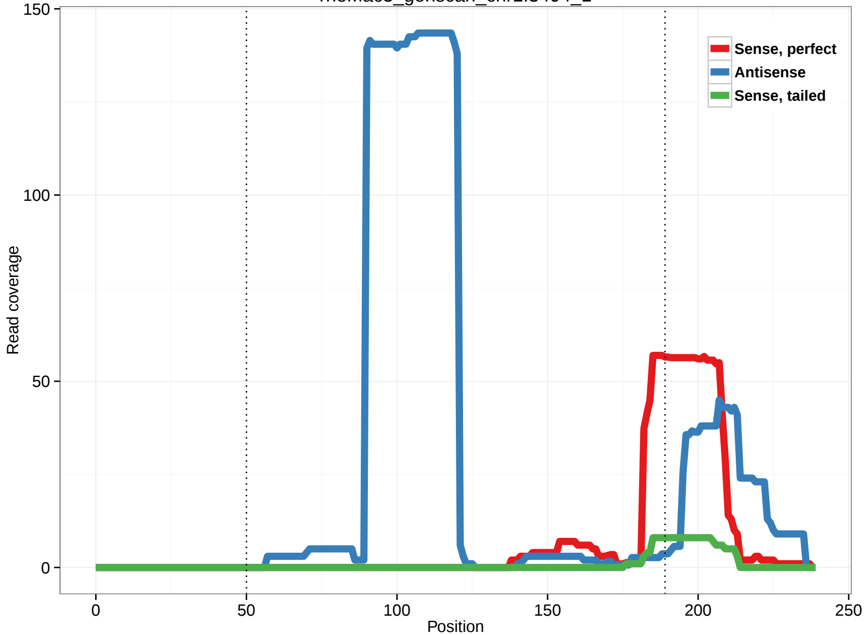
rheMac3_genscan_chr1.3404_1
