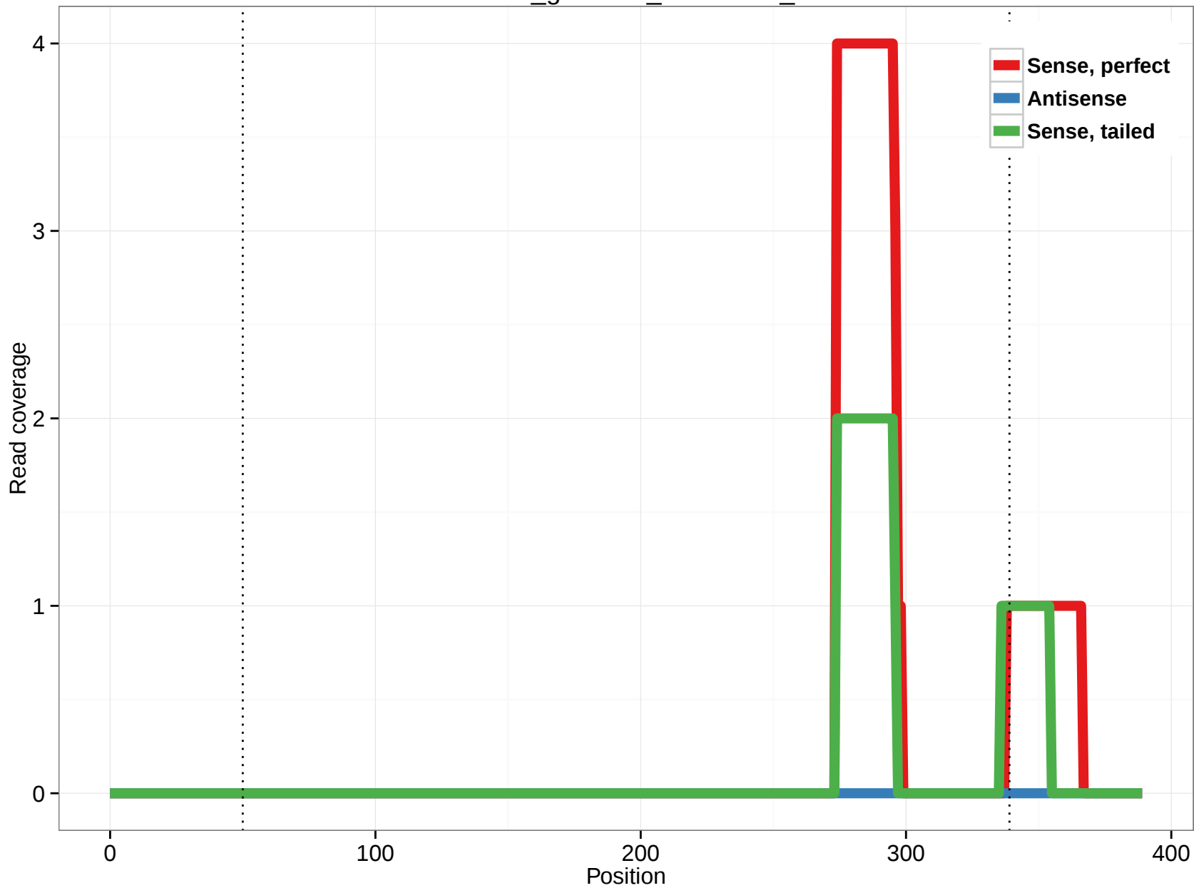
rheMac3_genscan_chr1.3395_14
