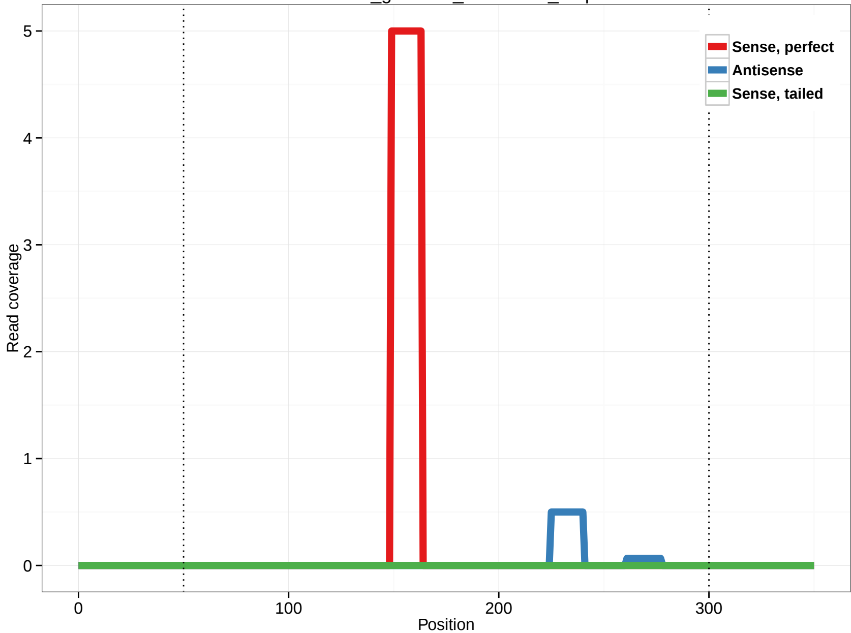
rheMac3_genscan_chr1.3381_1.5p
