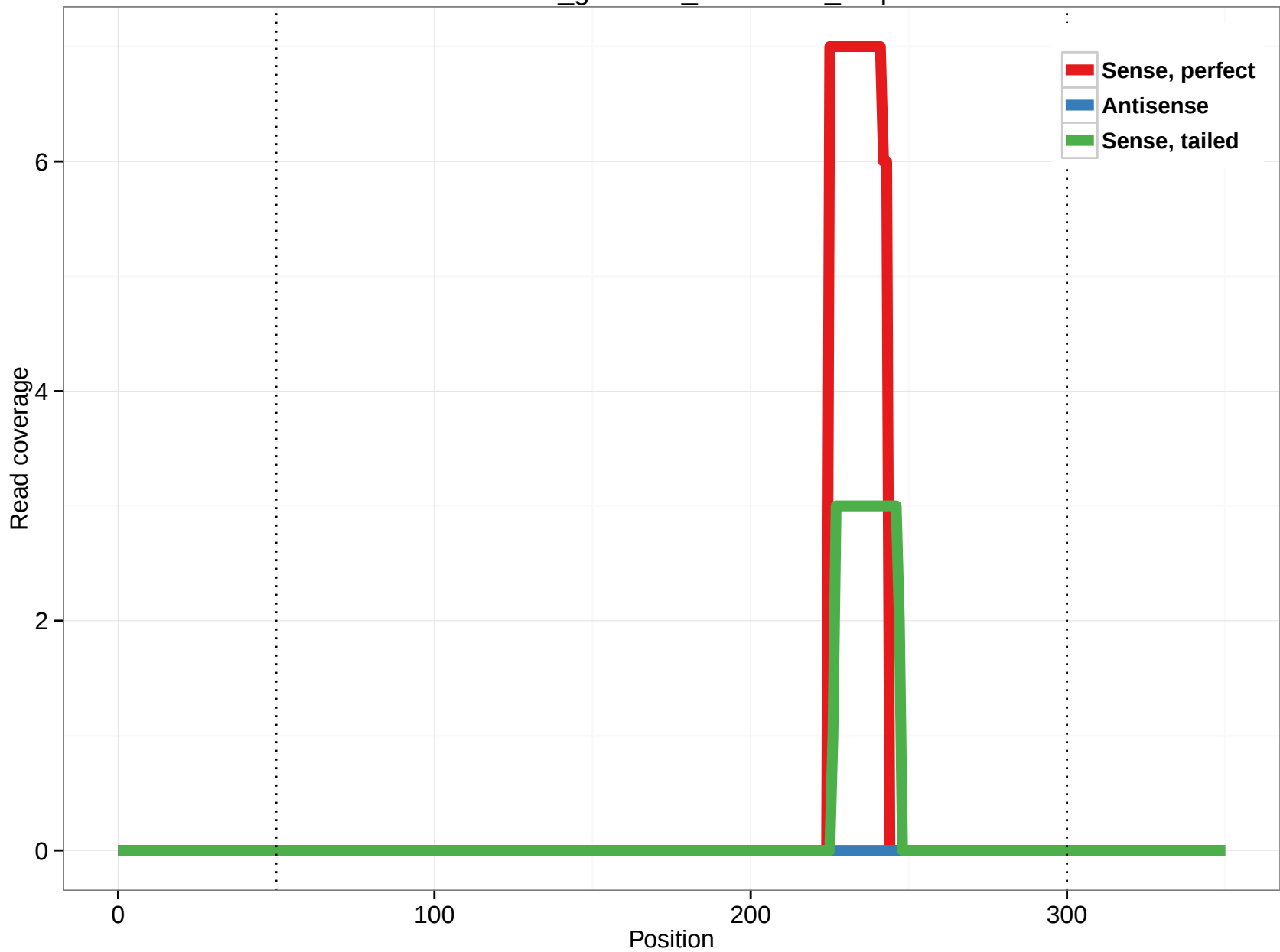
rheMac3_genscan_chr1.3289_1.5p
