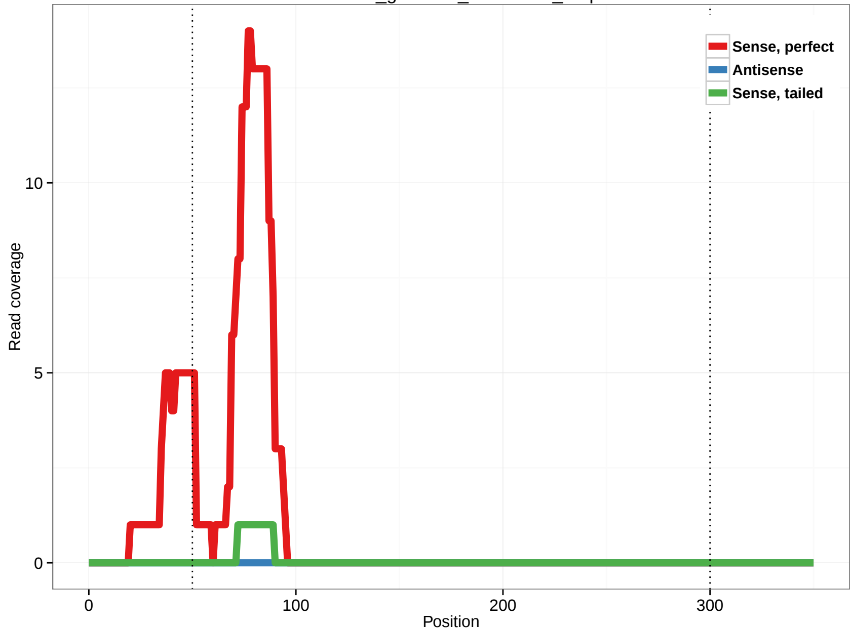
rheMac3_genscan_chr1.3178_0.5p
