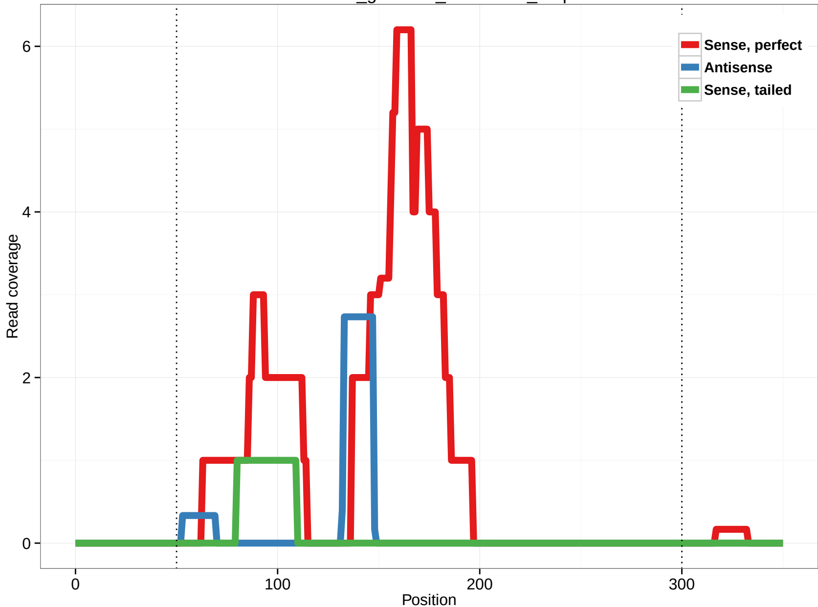
rheMac3_genscan_chr1.3108_8.5p
