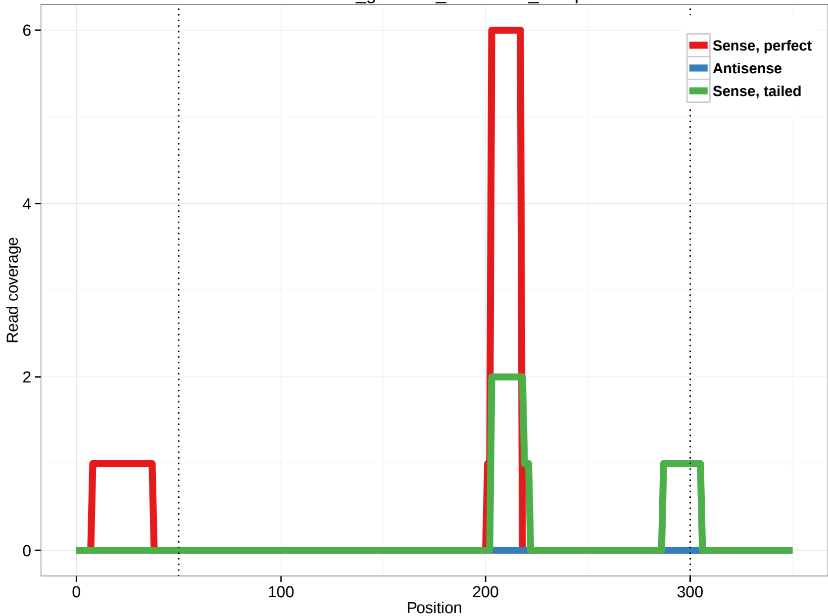
rheMac3_genscan_chr1.3050_10.5p
