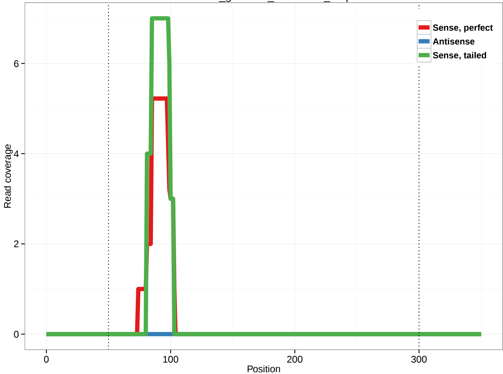
rheMac3_genscan_chr1.3043_6.5p
